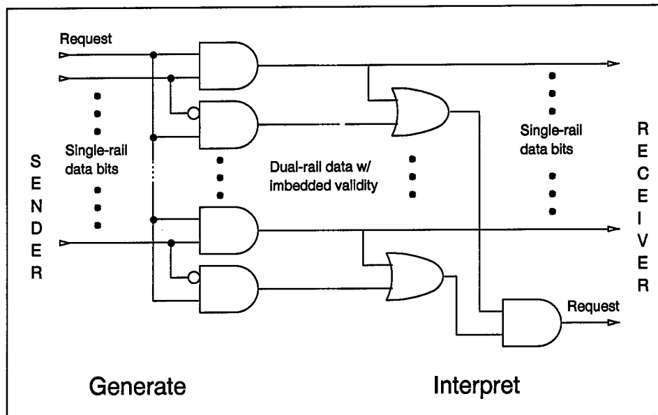
Figure 3.4 Dual-Rail Data Generation and Interpretation
