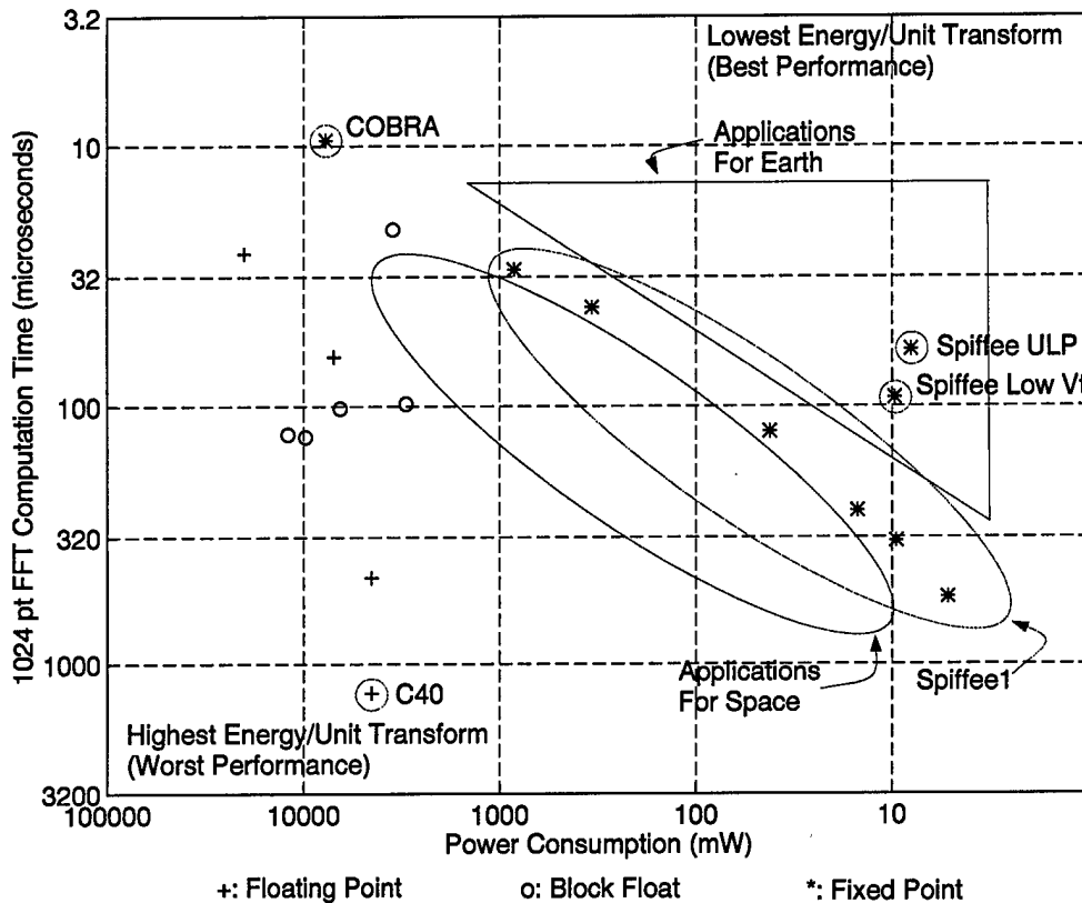
Figure 2.1 Comparison of Existing FFT Processors
