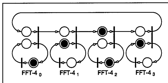
Figure 4.4 Expander Petri-net
