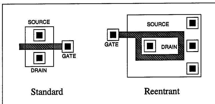
Figure 3.6 N-FET Designs
