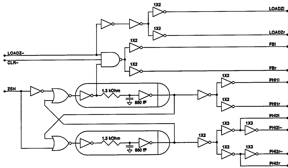
Figure 5.24 Two Phase Pulse Generator
