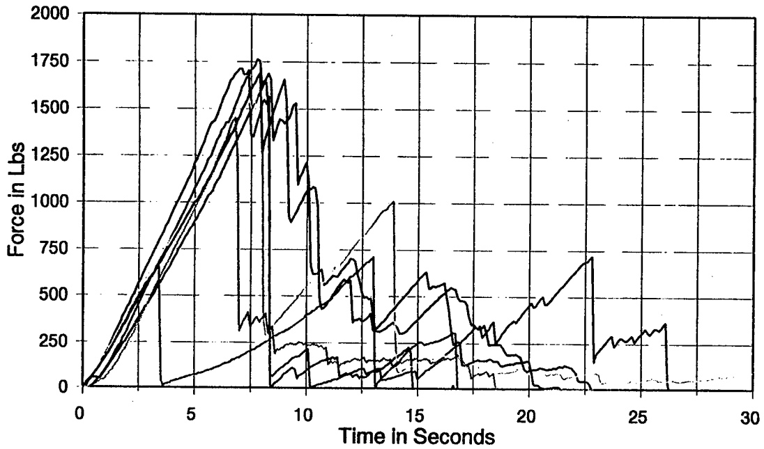
Figure 5 Symmetrical Girt Loading Test Results
