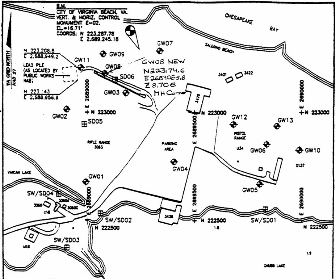
Figure 5: Groundwater Monitoring Well Survey
