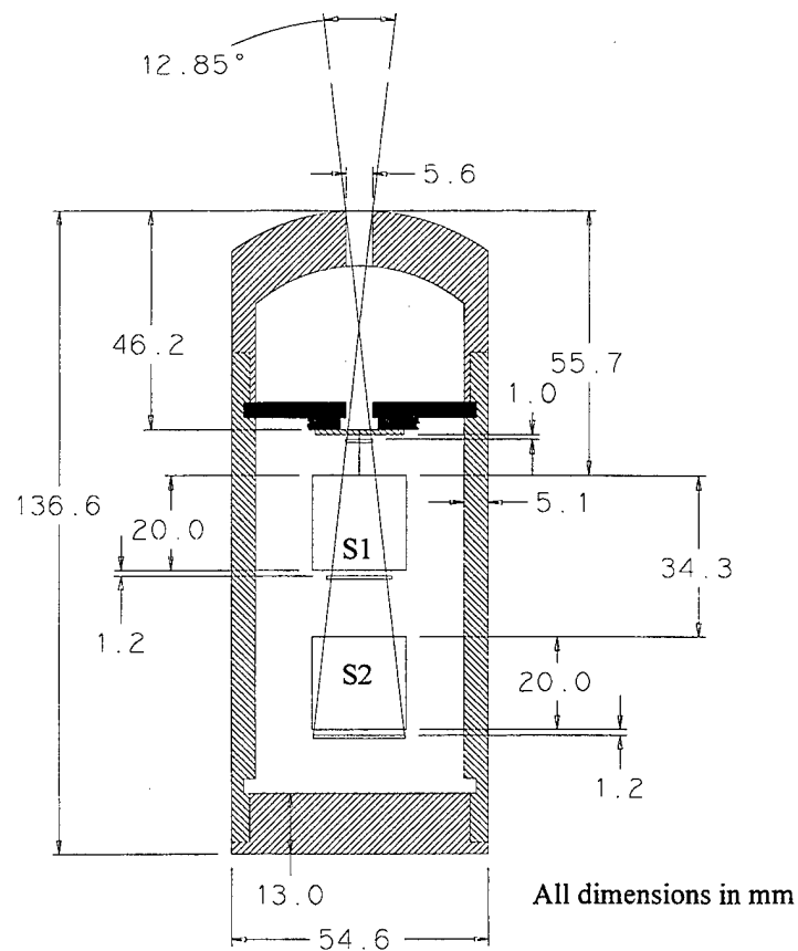
Figure 1. Cross section diagram of the HEP EM sensor head.
