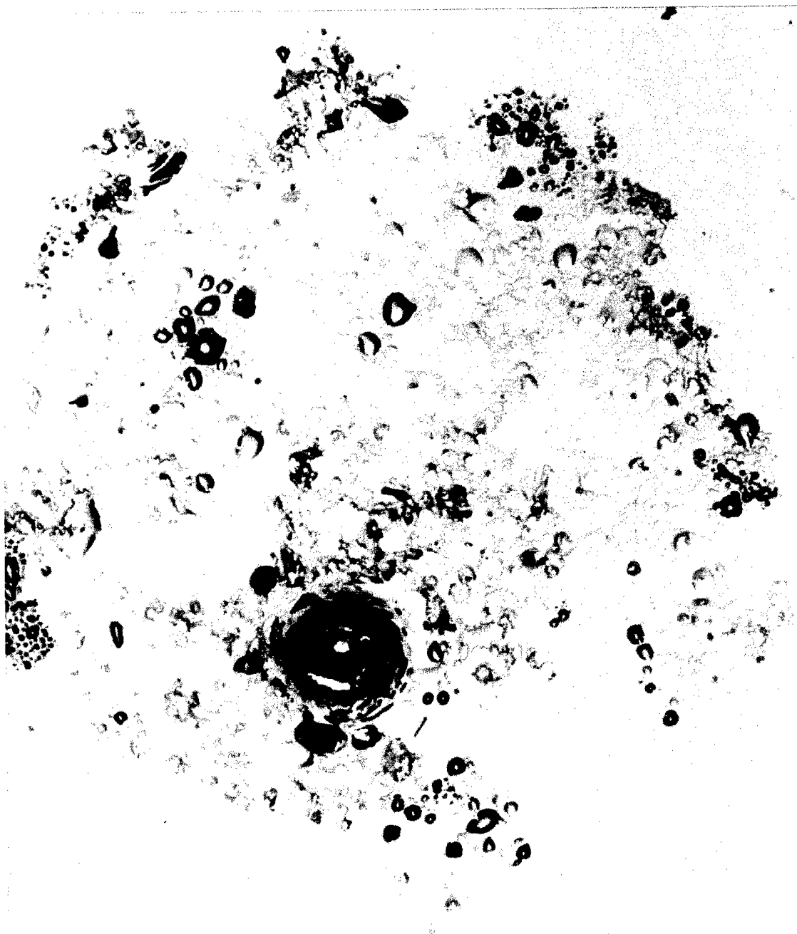
Figure 4.4.2.2 -3. An Impact Crater With an Expanded, Asymmetric Area of Damage. The substrate is molybdenum with a \text{Cr/Ag/ThF}_4 coating. (Photograph courtesy of The Aerospace Corporation)
