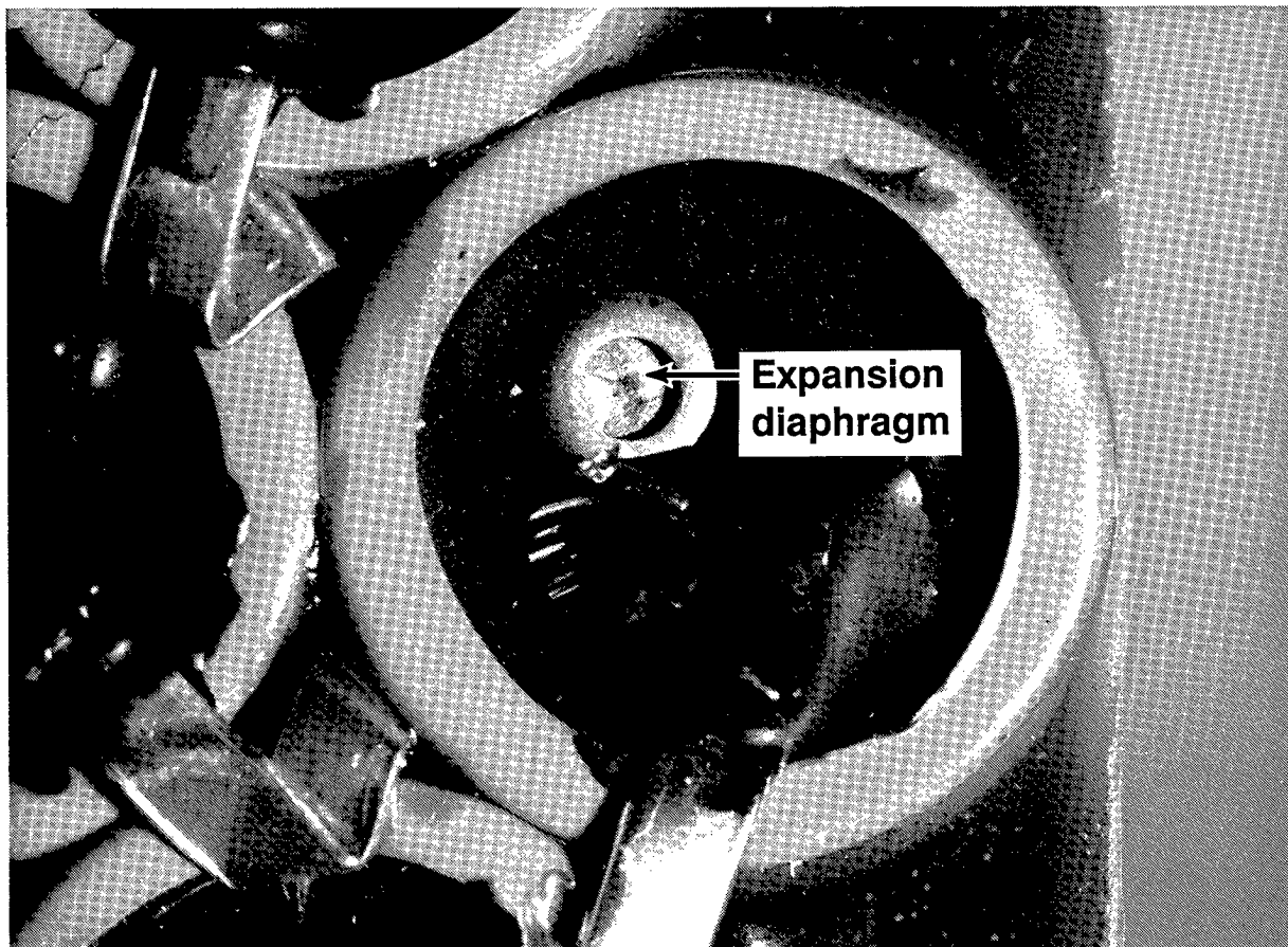
Figure 4.2.3.2-3. LiCF Cell
