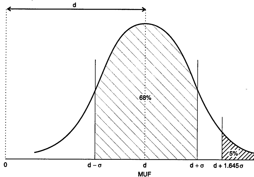
Figure b. Expected probability distribution of MUF measurements from the same system as figure a) in the event that amount "d" of nuclear material has been diverted. Measurements of missing or unaccounted-for material are most likely to be near d, falling between d-\sigma and d+\sigma 68 percent of the time.
