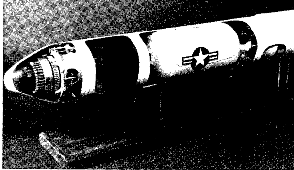
Cutaway view of the ASAT missile, showing MV in nose cone atop ALTAIR upper stage on SRAM (Short Range Attach Missile) booster.
