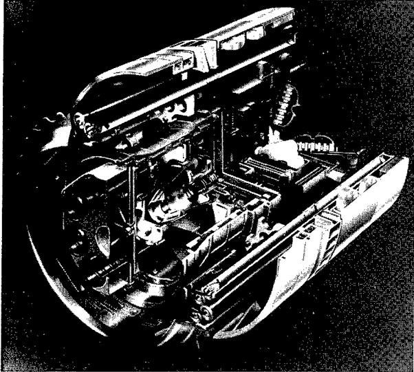
Cutaway view of the ASAT missile warhead (the Miniature Vehicle).
