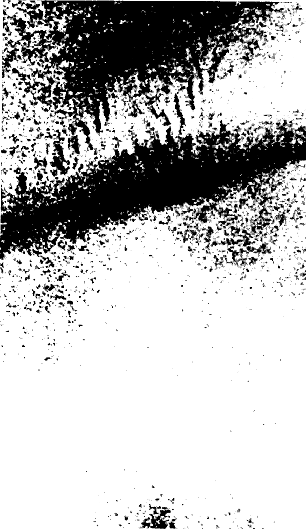
Left, imagery of Atlantic Ocean waves obtained by the Soviet Kosmos 1500 Oceanographic Research Satellite in 1983.
