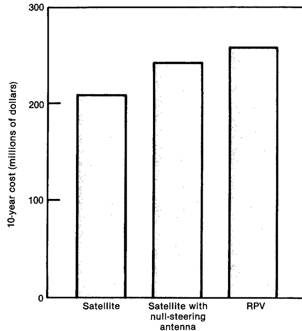
Figure 4-13.—Cost Comparison: Satellite and RPV Relays for Single-Channel UHF Tactical Theater Communications
