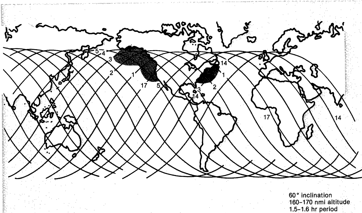
Figure 3-1.—Ground Track of Soviet Radar Ocean Reconnaissance Satellite
