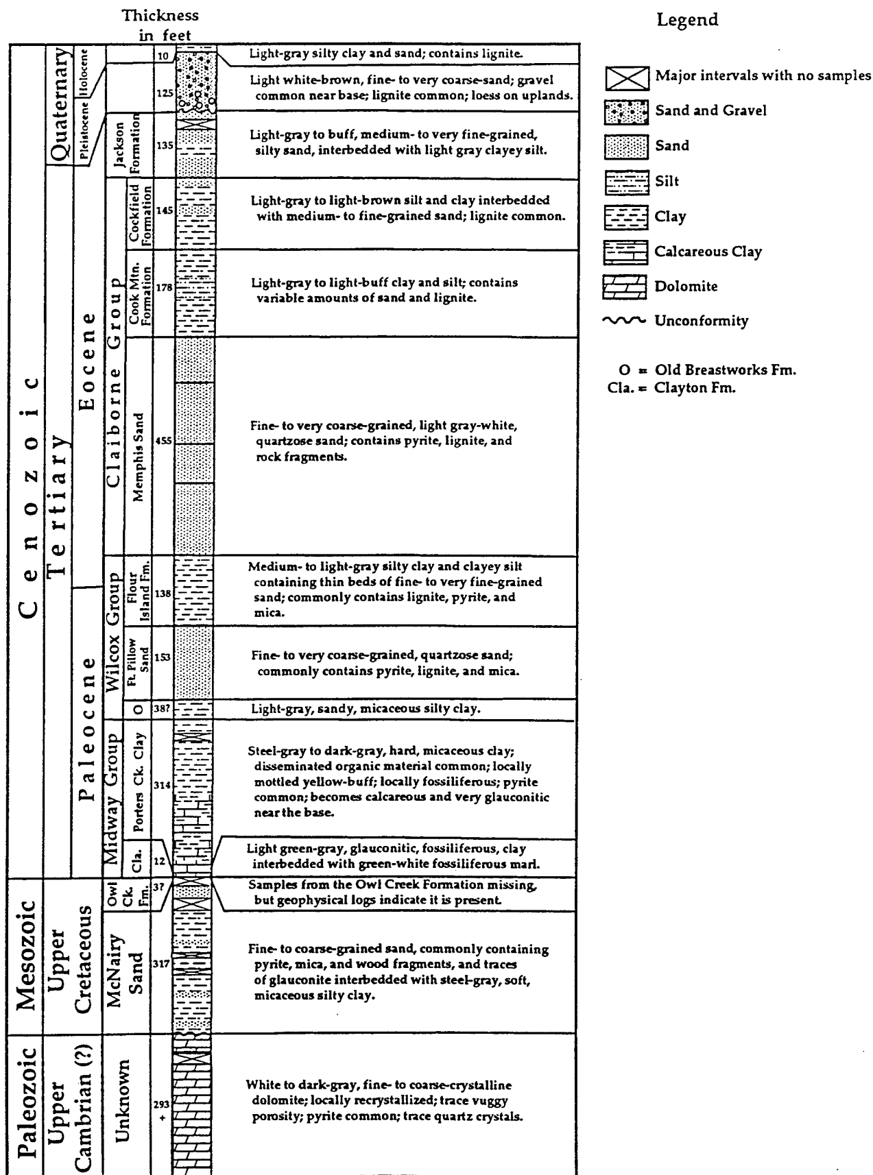
Figure 15. Columnar stratigraphic section of the New Madrid test well X-1. From Purser, 1996.
