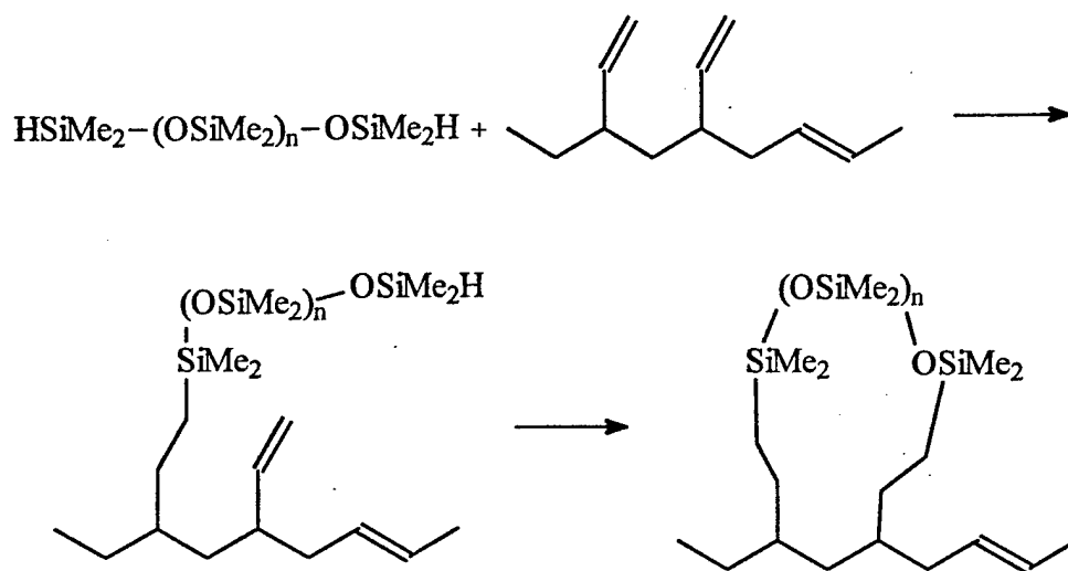
Scheme 1. Side-loop formation.
