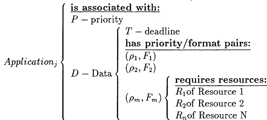
Figure 30. Mapping of mathematical terms to an application.
