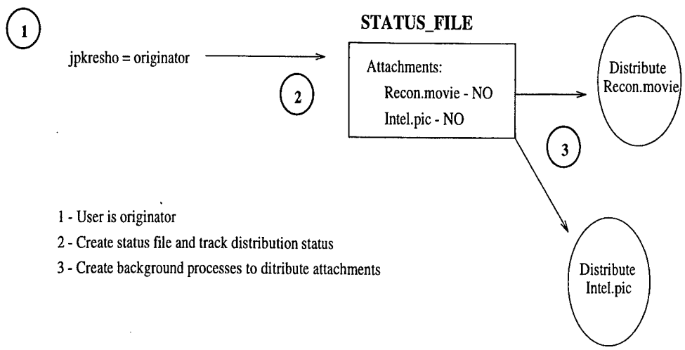
Figure 11. Creation of status file and distribution of attachments.
