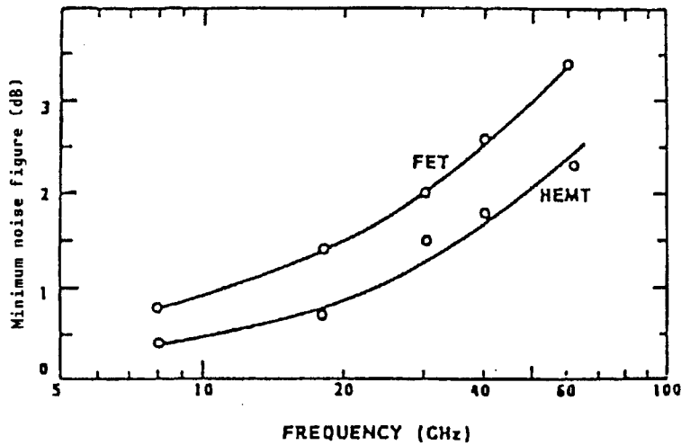
Figure 2.5 Comparison of Noise Indices for FET and HEMT at 0.25 \mu\text{m}
