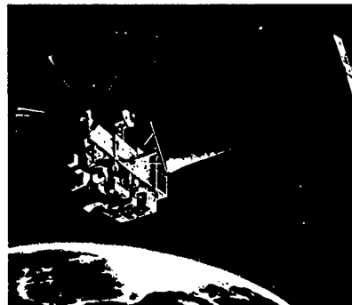
▲ Observation of change the global environment by the Advanced Earth Observing Satellite (ADEOS)
