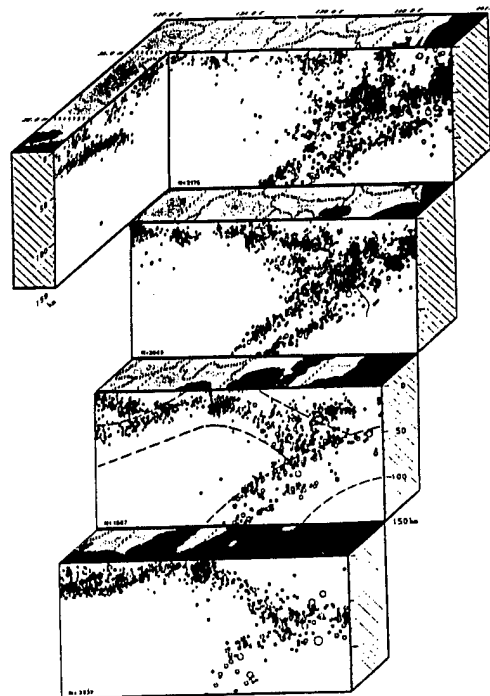
Vertical cross section of earthquake hypocenters down to 150 km underground in the Kanto and Tokai Districts (from the data obtained for the recent 5 years)
