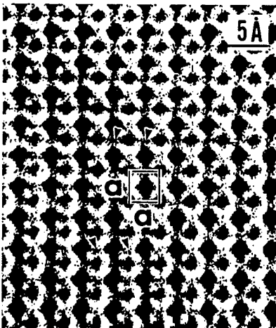
▲ Yttrium high temperature super conductor taken by electro-microscope (Black dots pointed by arrows indicate oxygen atoms, the first successful observation done in the world)
