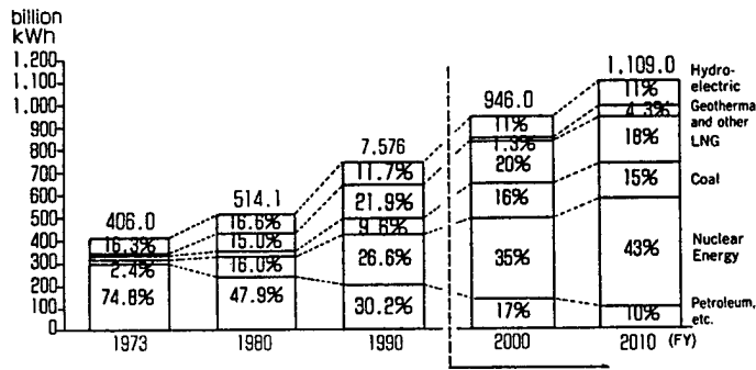
Target of electric power supply (Interim report of Electric Utility Industry Council (June, 1990))
