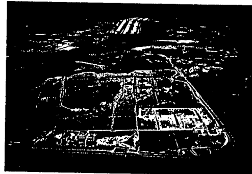
Air Photograph of Nuclear Fuel Cycle Facilities
