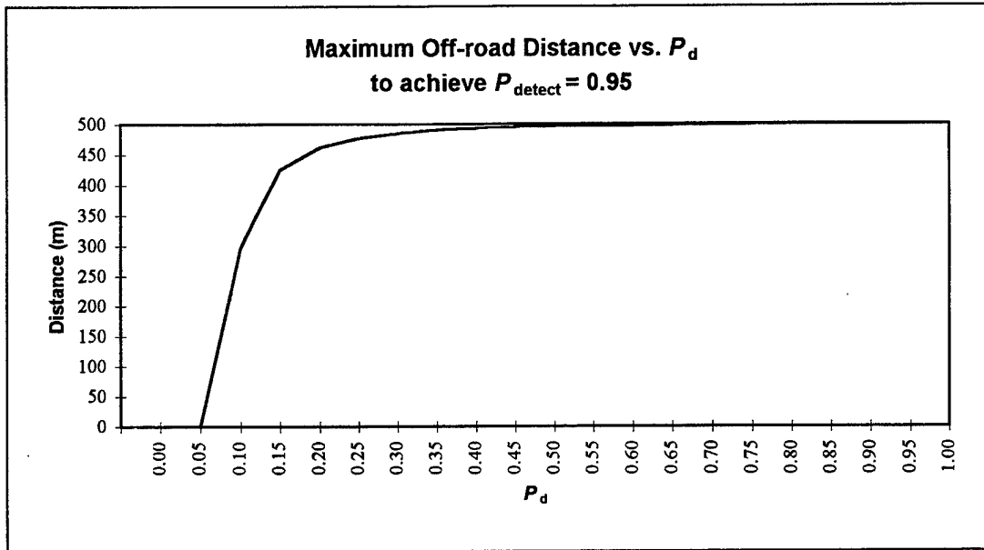
Figure 2.5 - Maximum Off-road Distance vs. P_d
