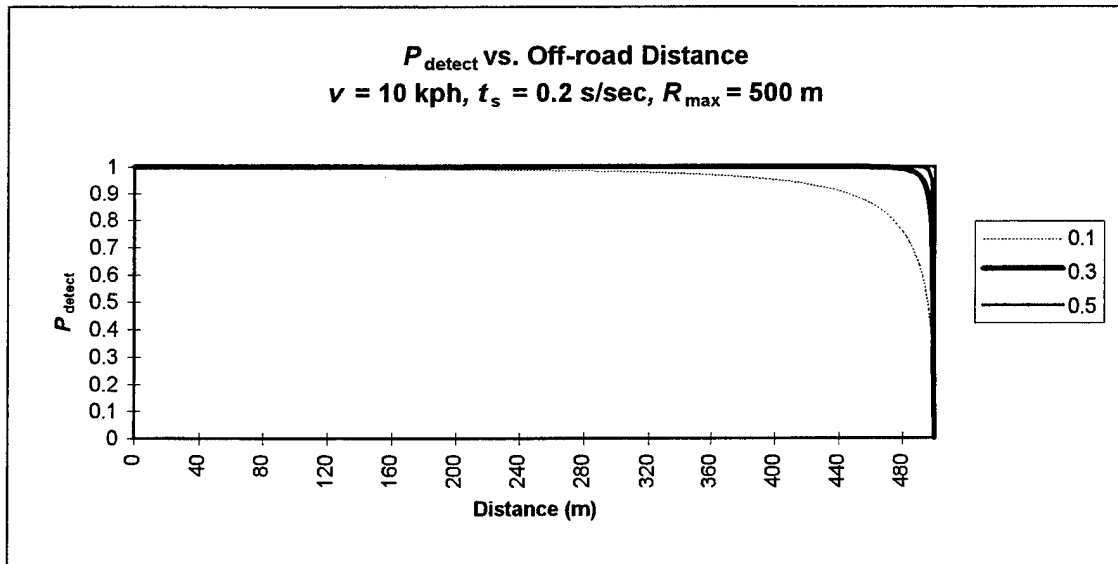
Figure 2.4 - P_{\text{detect}} as Function of Off-road Distance
