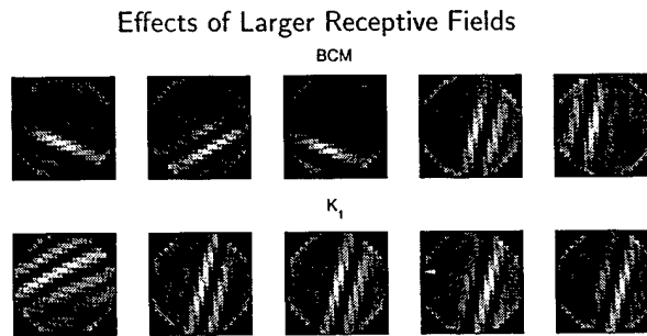
Figure 7: Large receptive fields using DOGED image input, obtained from the Quadratic BCM learning rule and the rule maximizing the multiplicative form of kurtosis.
