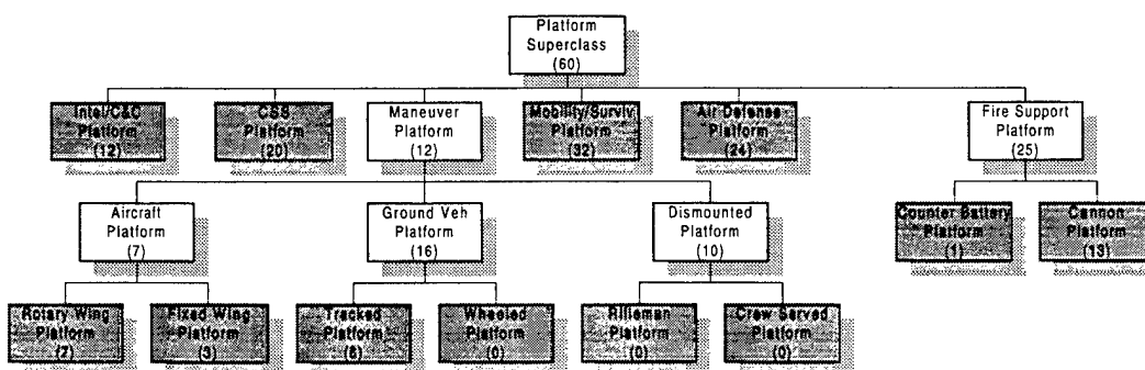
Modified Platform Class Hierarchy
