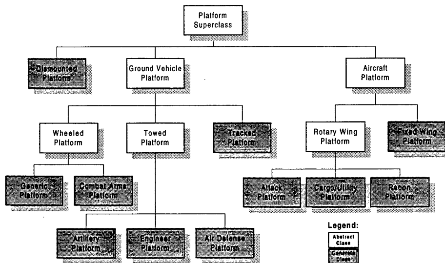
Figure 2. Platform Class Hierarchy.
