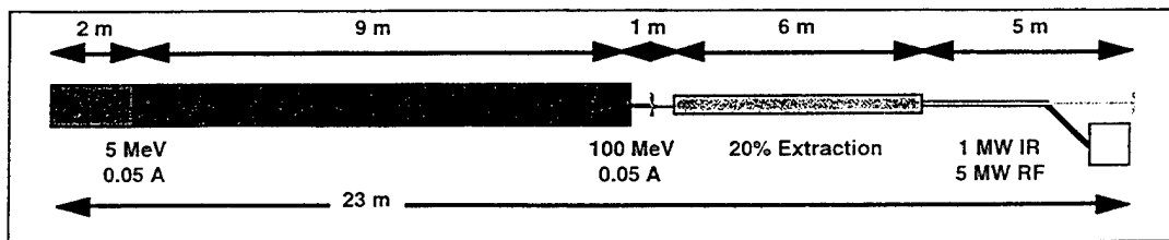
Figure 9. This is a conceptual MW class amplifier FEL. From [Ref. 15].
