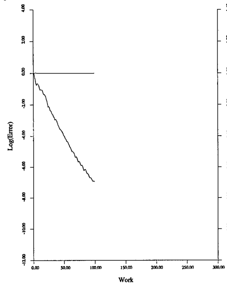
Figure 23b: Convergence.
