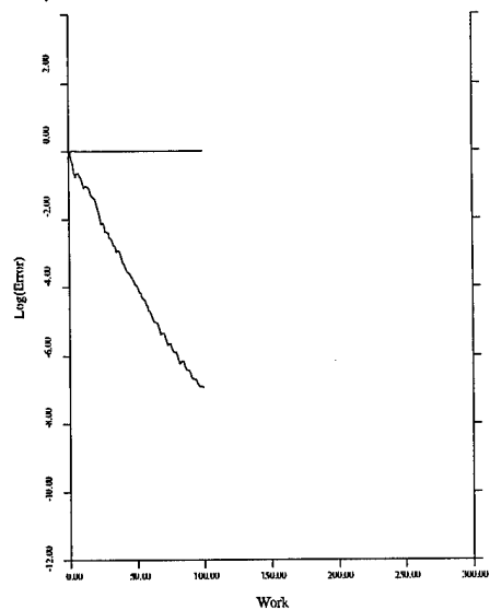
Figure 23b: Convergence.
