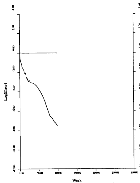
Figure 21b: Convergence.
