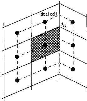
Figure 6a: Cell-centered scheme. \sigma_{ij} evaluated at vertices of the primary mesh
