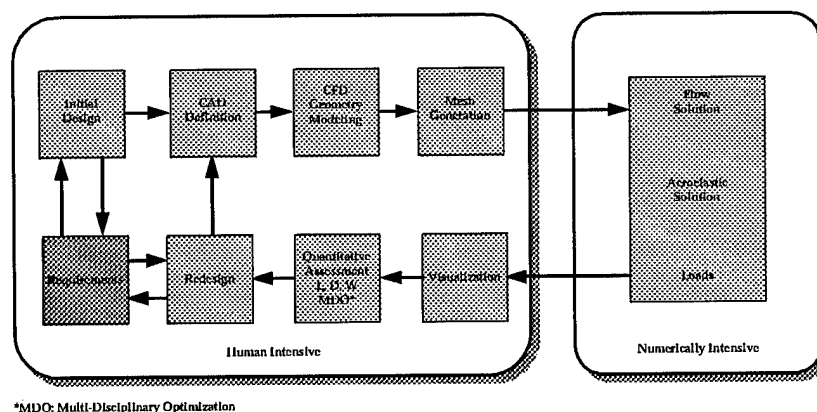
FIG. 18. Concept for a numerical wind tunnel.
