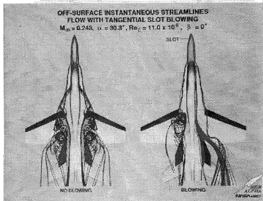
FIG. 20. Navier-Stokes Predictions for the F-18 Wing-Fuselage at Large Incidence
