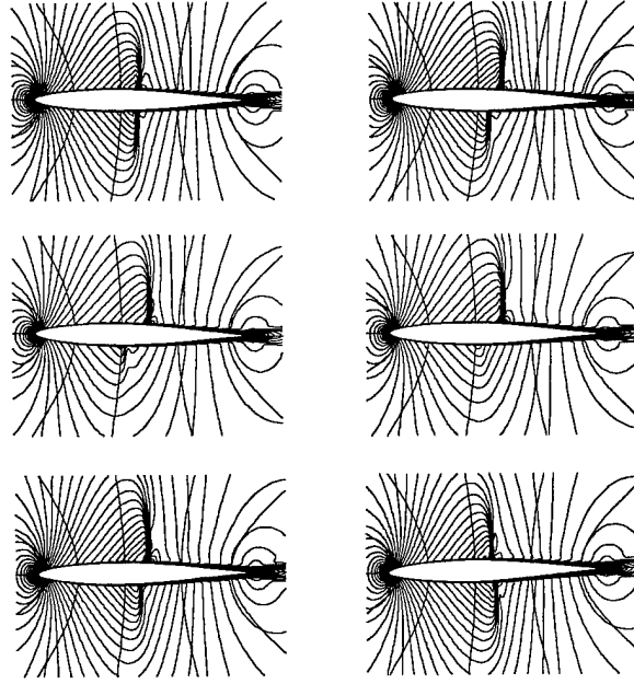
FIG. 14. Mach Number Contours. Pitching Airfoil Case. Re = 1.0 \times 10^6 , M_\infty = 0.796 , K_c = 0.202 .
