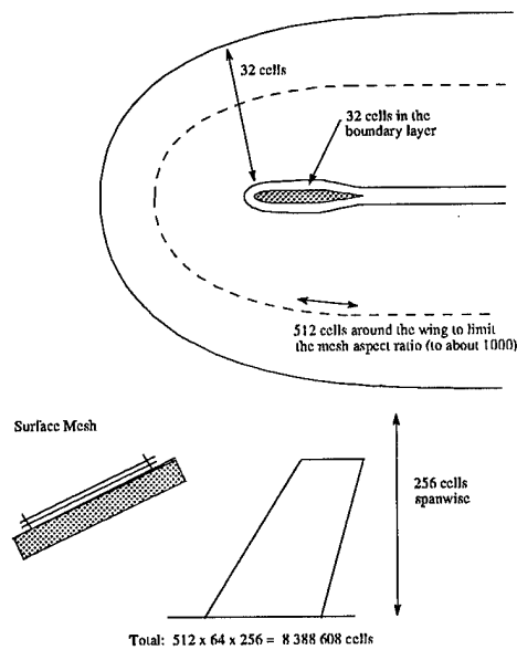
FIG. 2. Mesh Requirements for a Viscous Simulation
