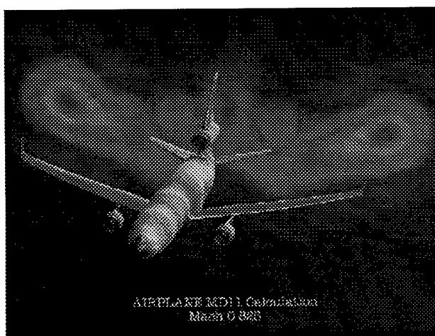
FIG. 12. Computed Pressure Field for a McDonnell Douglas MD11
