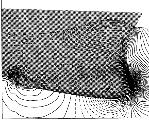
FIG. 17. Pressure Contours in the Bow Region
