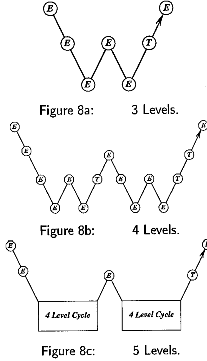
FIG. 8. Multigrid W-cycle for managing the grid calculation. E, evaluate the change in the flow for one step; T, transfer the data without updating the solution.
