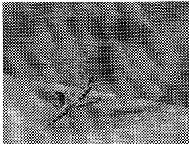
FIG. 11. Pressure Contours and Sonic Boom on a Representative HSCT Configuration
