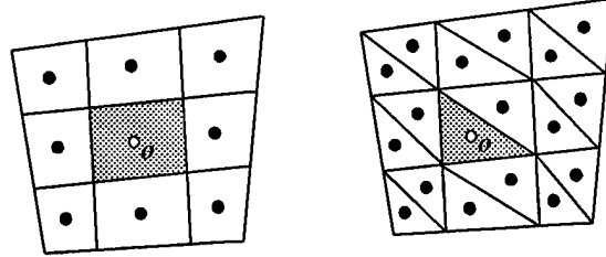
Figure 3a: Cell Centered Scheme.
