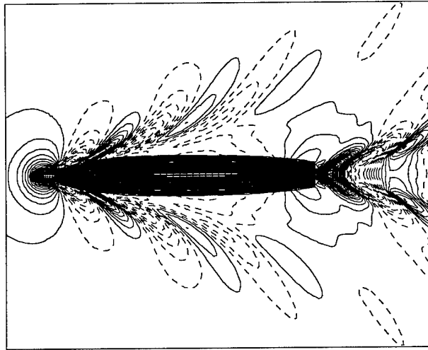
FIG. 15. Contours of Surface Wave Elevation for a Combatant Ship
