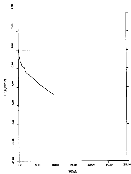
Figure 22b: Convergence.
