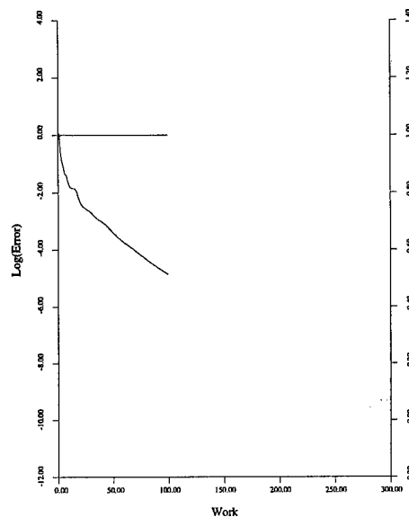
Figure 22b: Convergence.
