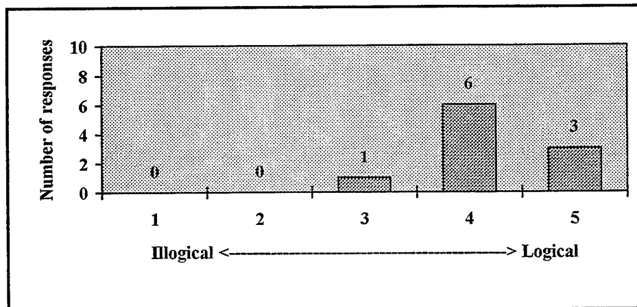
Figure 4.22. Information Arrangement
