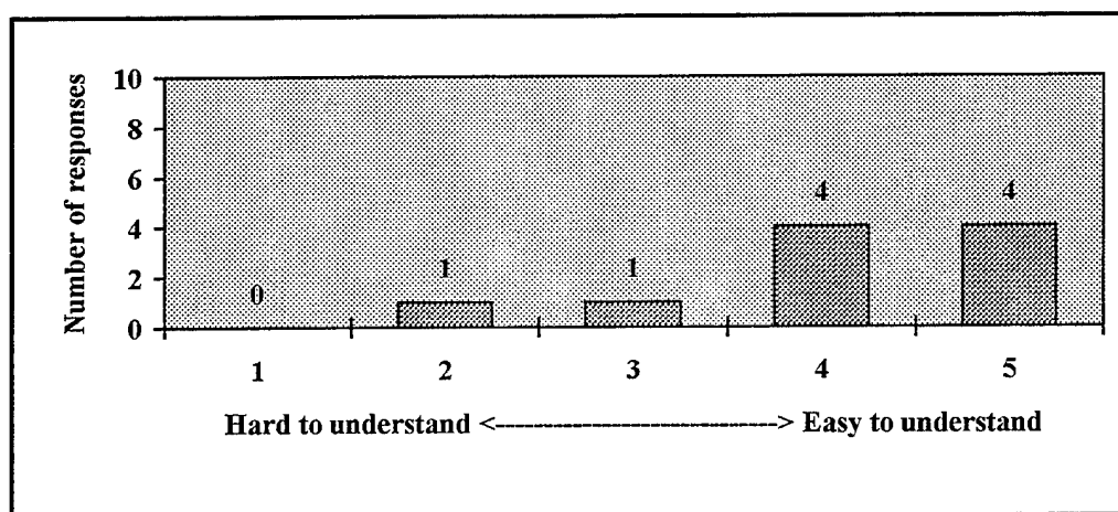
Figure 4.20. Graphical Displays
