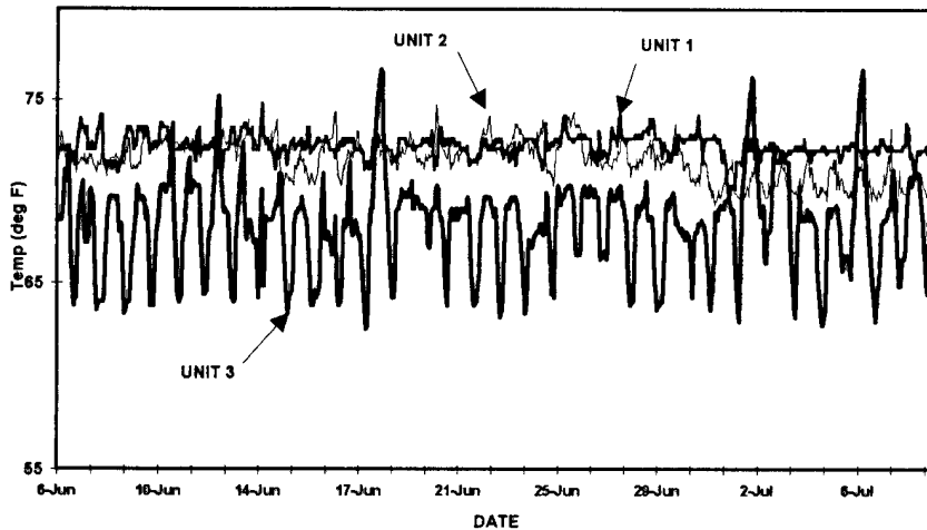
RETURN AIR TEMPERATURES, JUNE 1996 FT HOOD GHP TEST UNITS
