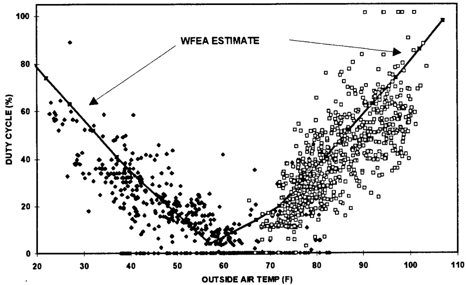
DUTY CYCLE VS AIR TEMP, FT. HOOD UNIT 1 GHP, JULY & DECEMBER, 1995
