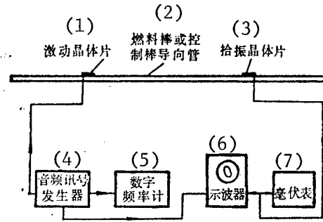
Figure 2. The System for Testing the Original Frequencies of the Fuel Rods and the Guiding Pipes
