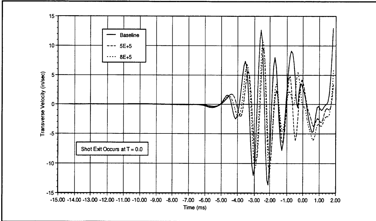
Figure 11. Transverse velocity of gun muzzle (S/N 17343) using base and softer spring constants of forward bourrelet.
