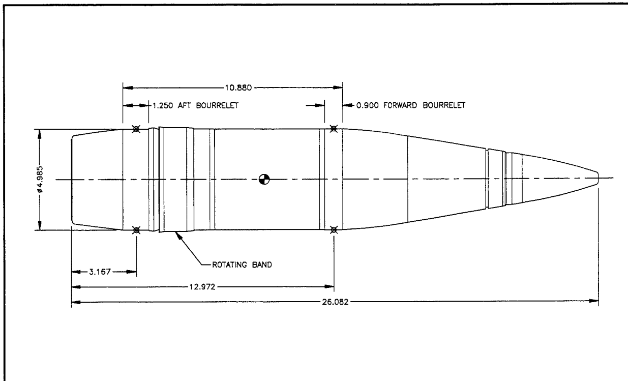
Figure 1. Mk 64 5-in projectile.
