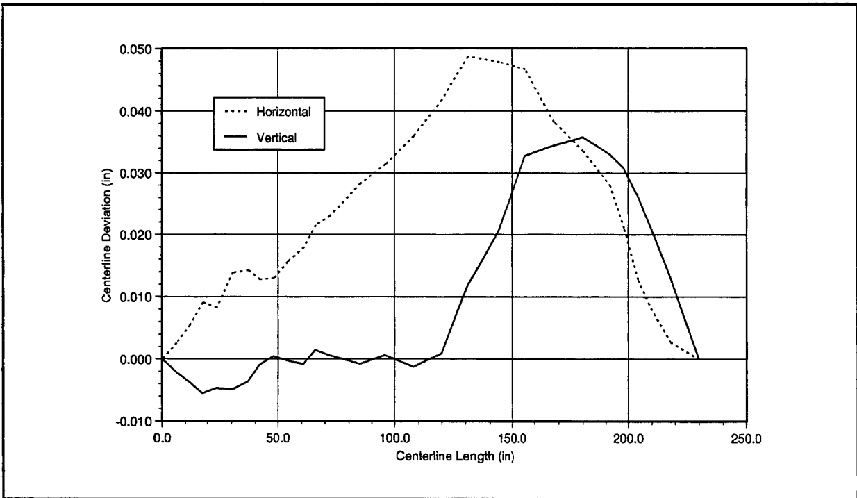
Figure 3. Gun barrel S/N 518 centerline data.
