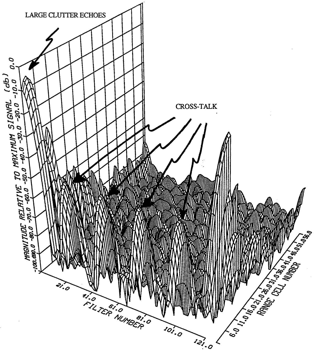
Fig. 5 - Air Channel ambiguity diagram showing large clutter echoes and Surface Channel cross-talk when using the current radar configuration without the diplexer. This data was collected at Wallops Island while looking along the beach.
