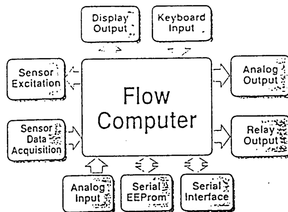
GF Series Top Level Block Diagram
