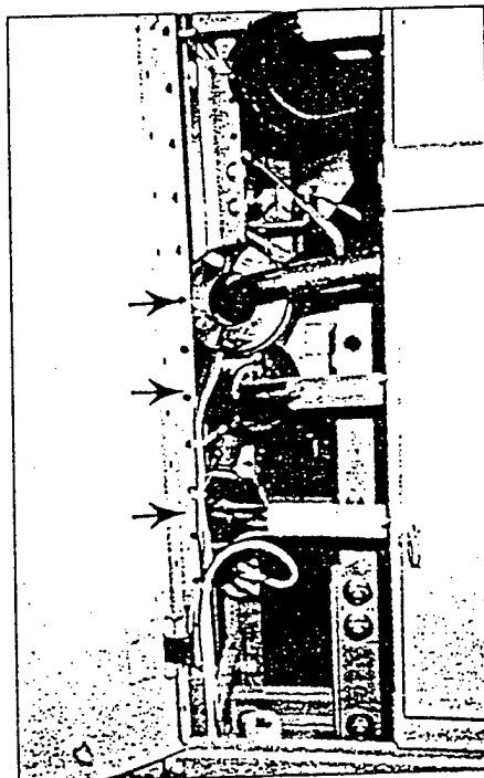
Three CTs (arrows) were installed on the load side phase conductors for one of the molding hall power monitors.
