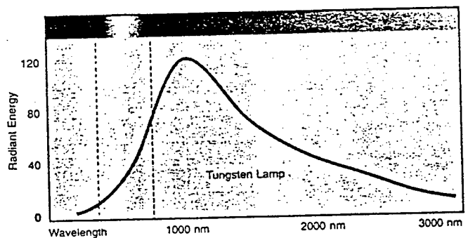
Figure 2. Tungsten lamp radiating at 3000 deg. K. Very little energy falls within the visual region, most is in the infrared.
