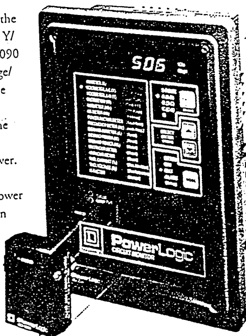
An I/O module and either a voltage/power module, or a control power module can mount on the back of the circuit monitor.
