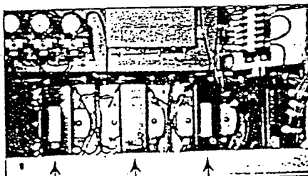
Three existing PTs (arrows) were replaced with identically-mounted units with different ratios.
