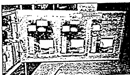
Rear view of three molding hall power feeder monitors shows input connections for CTs and PTs, along with shielded twisted pair cables, running to terminal strips just inside existing switchgear.
