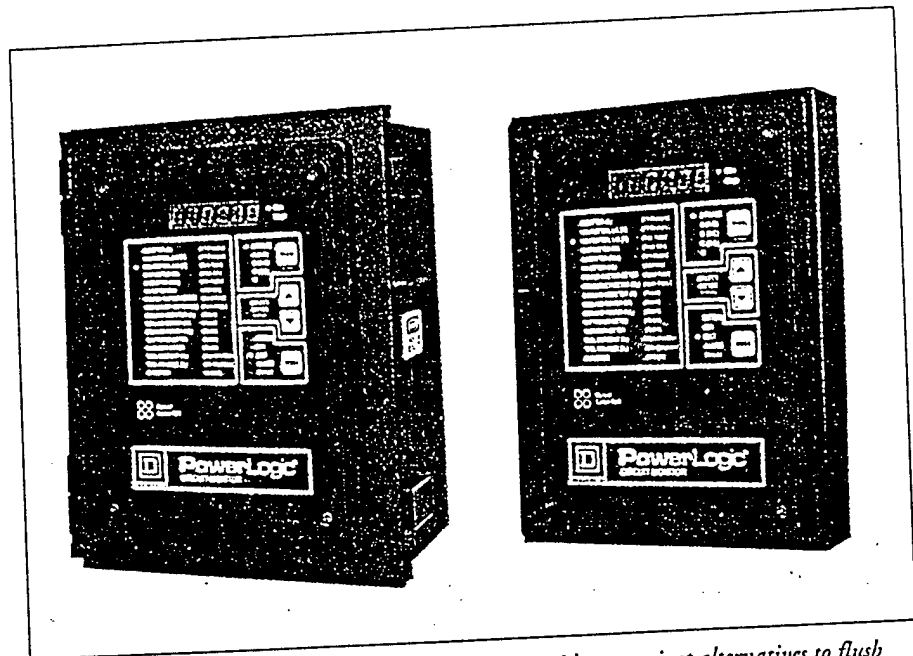
The 3090 SMA-220 (left) and the 3090 CMA-100 provide convenient alternatives to flush panel mounting.
