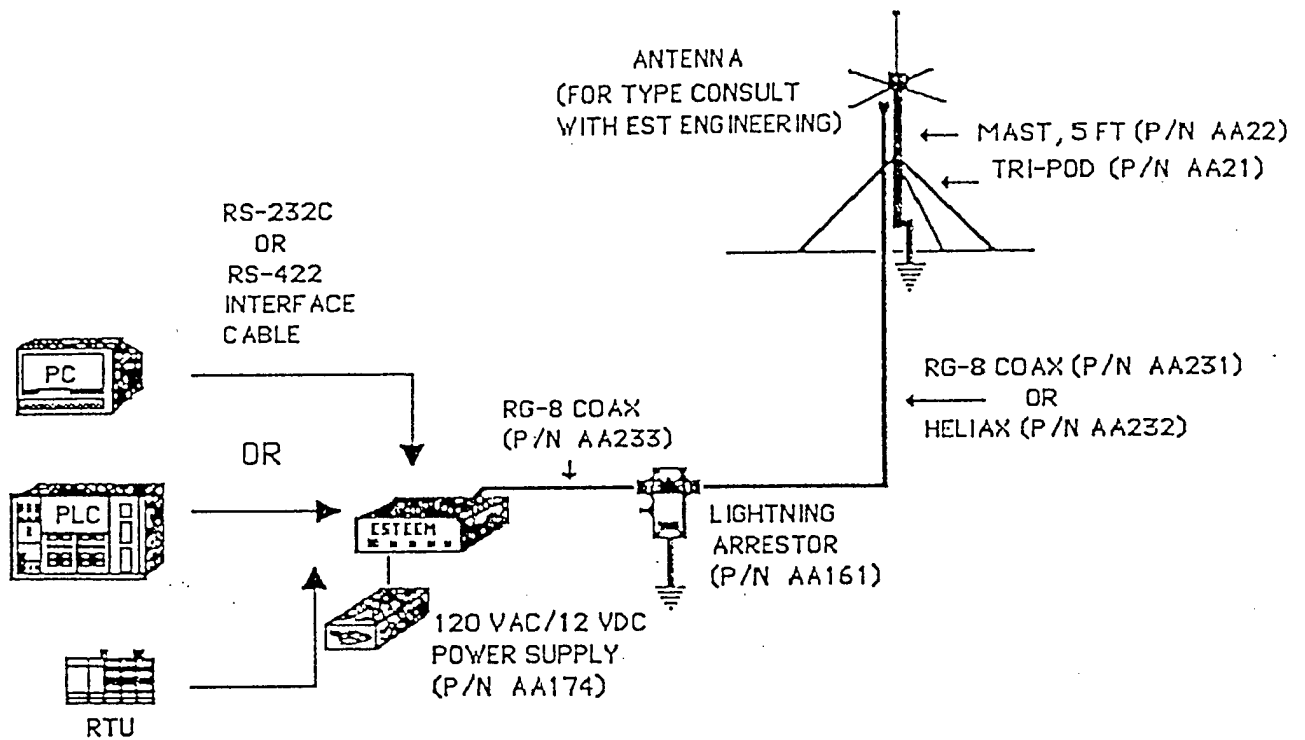
TYPICAL NODE BLOCK DIAGRAM
