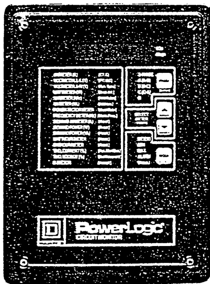
POWERLOGIC Circuit Monitor
