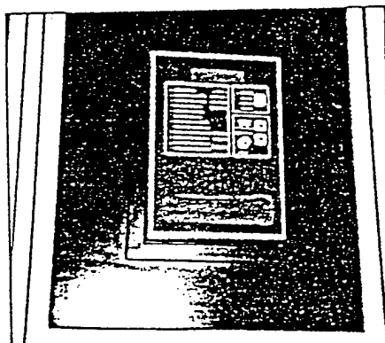
Front of existing panel has new monitor installed in faceplate, with painted sheetmetal panel installed above it.
