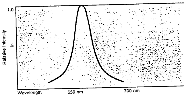
Figure 1. Typical spectral distribution of LED at 660 nm. Note the peak at the specific wavelength, and the rapid fall-off.
