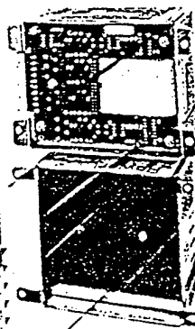
An I/O module and either a voltage/power module, or a control power module can mount on the back of the circuit monitor.
