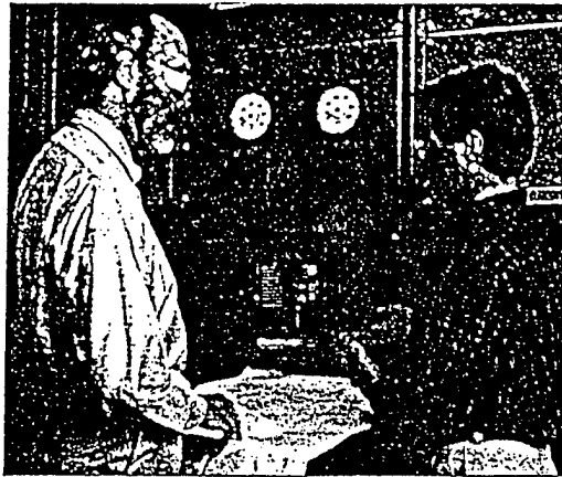
Circuit monitors in the plant, easily retrofit into existing gear, collect electrical data needed for better decisions.
