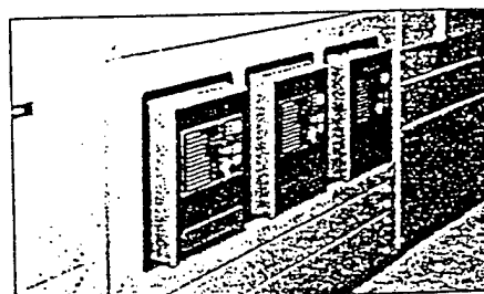
Three new monitors are installed in lower front panel of existing switchgear and monitor three molding hall feeders. Panel front was measured and cut to accept monitors. Feeder overcurrent protective devices (OCPDs) are located above and to the right of the monitors.
