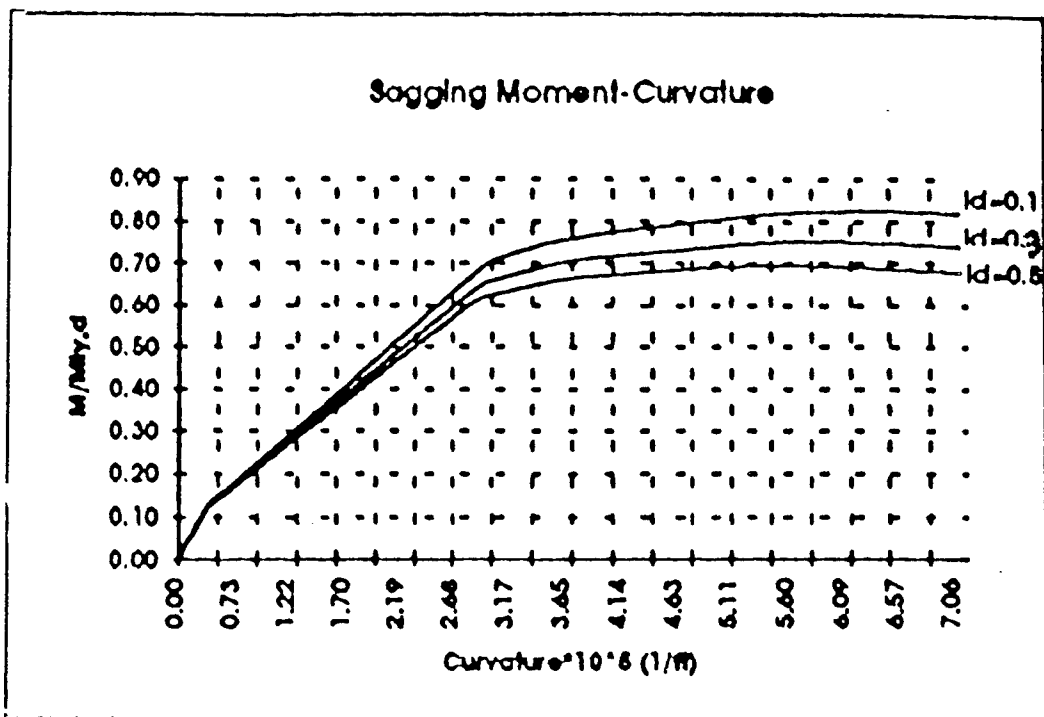
Figure 4.1.7 Tanker Vertical Bending Moment-Curvature Relation (Referenced to Fully Plastic Moment)
