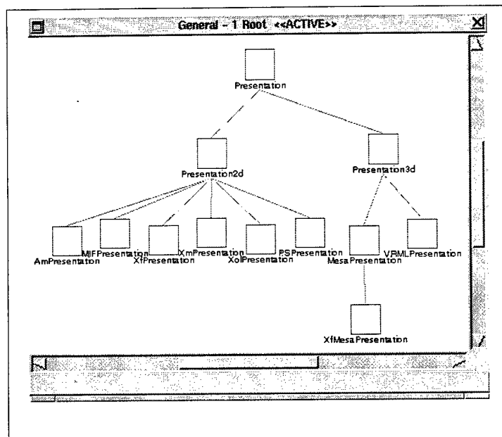
3-16 Presentation and its has_subclass Descendants
