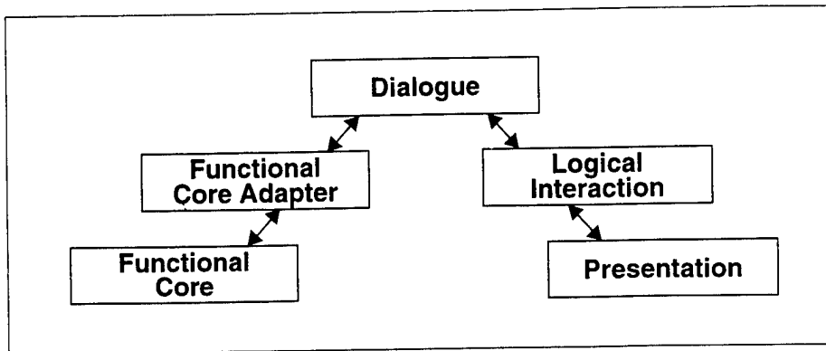
3-12 The Arch Metamodel of Interactive Software
