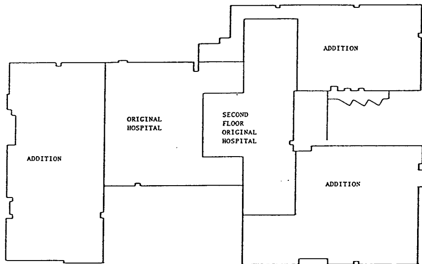
FIGURE 1. HOSPITAL LAYOUT
