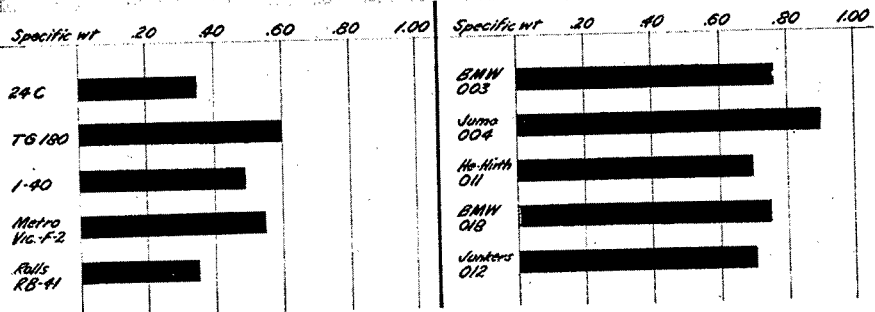
Figure 13 — Characteristics of Turbojets
