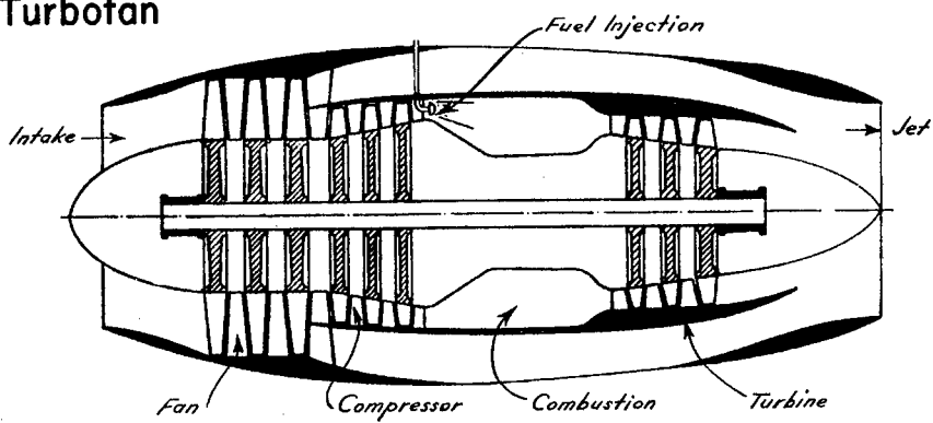
Figure 10-A — Various Propulsion Systems
