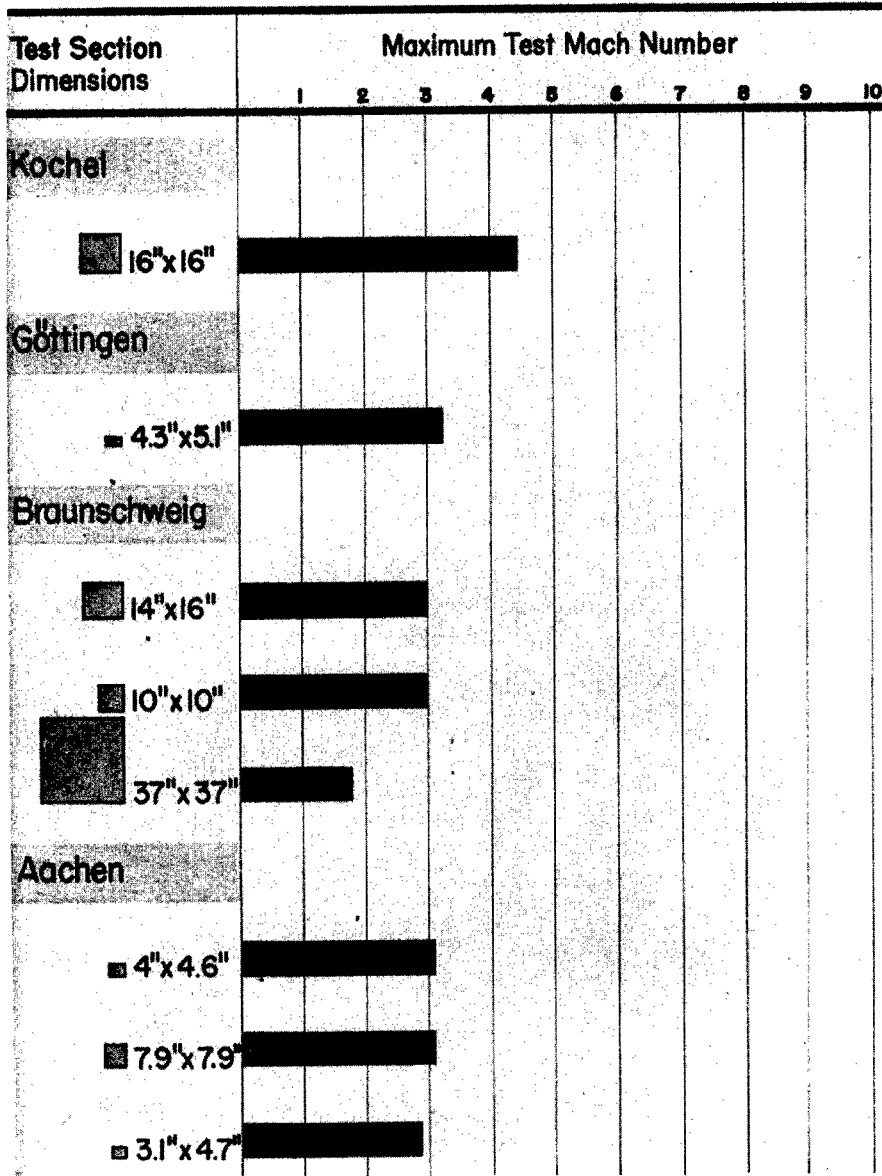
Figure 1 — German Supersonic Wind Tunnels (operation 1945)
