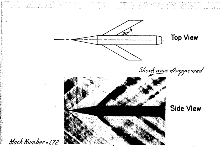
Figure 4 — Sweepback Effect on Shock Waves
