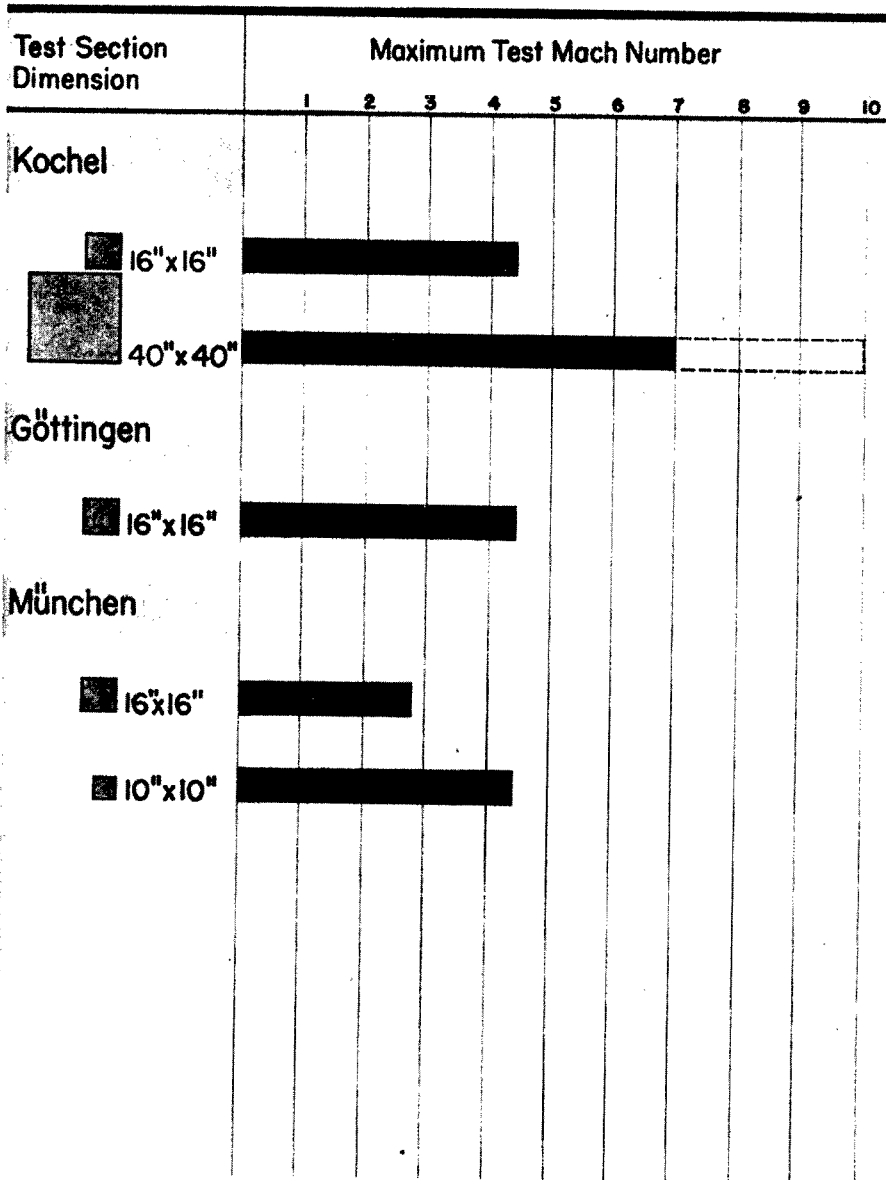
Figure 2 — German Supersonic Wind Tunnels (Construction 1945)
