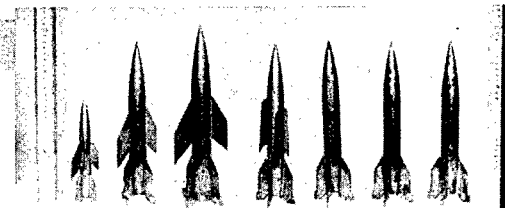
Figure 7 — Rocket Models for Supersonic Wind-Tunnel Tests
