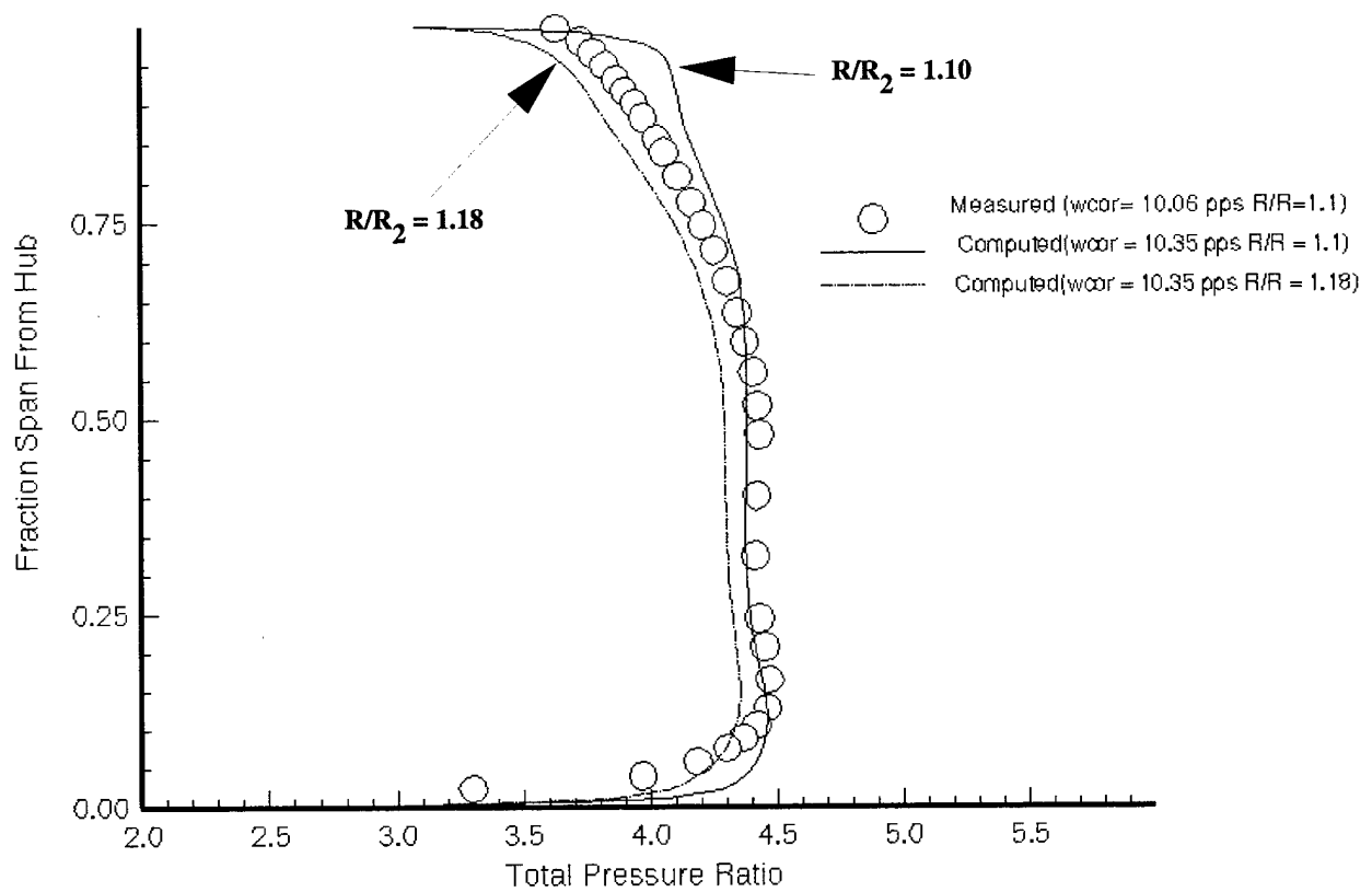
Fig. 5– Impeller exit spanwise distribution of circumferentially averaged total pressure at design operation (measurements at R/R_2 = 1.1 )
