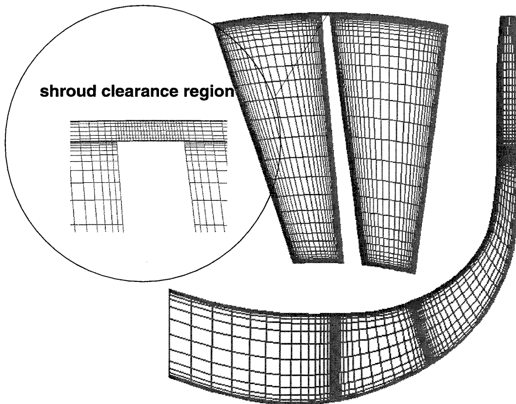
Fig. 2– Computational mesh of impeller discharging into vaneless diffuser showing closeups of impeller leading and trailing edges
