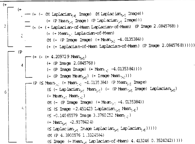
Figure 21.7 GP Switch-Filter Code.
