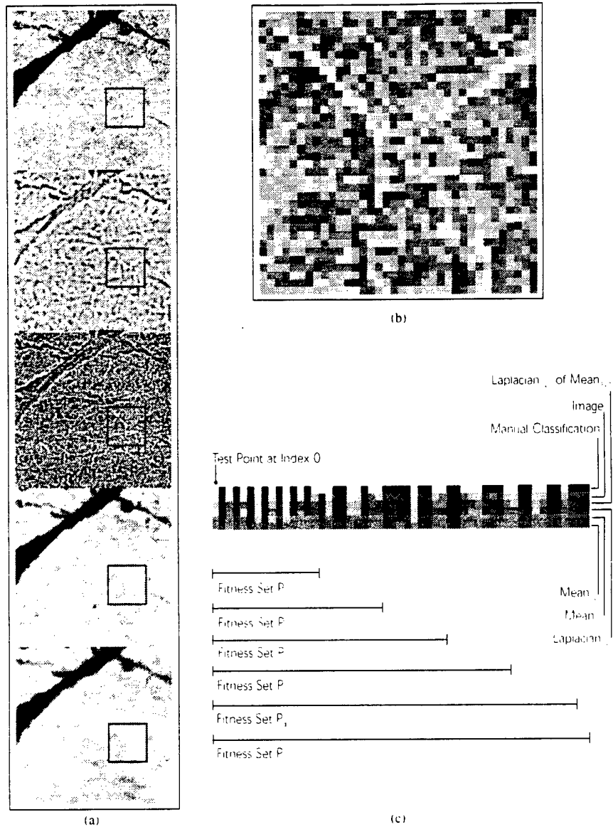
Figure 21.4 Fitness Set Construction. Starting from the upper left image: (a) 128 \times 128 pixel ERS-1 SAR image (April 23, 1992) and associated layers of texturally filtered images ( Laplacian_{i,j} of Mean_{i,j} , Laplacian_{i,j} , Mean_{i,j} , and Mean_{i,j} ). (b) Overlay of test point locations. White points indicate ridge guesses, while black points indicate background guesses. (c) Detail of Fitness Set. Each row corresponds to either a manual classification, image data, or layer of texturally filtered image data. Each column corresponds to a test point. Test points are loaded into an evaluation function by sets, starting from P_0 to P_n . Loading of a set is triggered by criteria that are set by a user.
