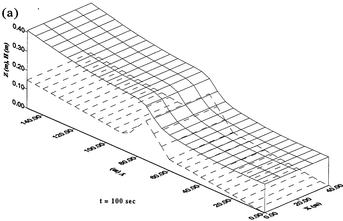
Figure 4.3a Simulated water stage at t = 100 \text{ sec} for Example 1A
