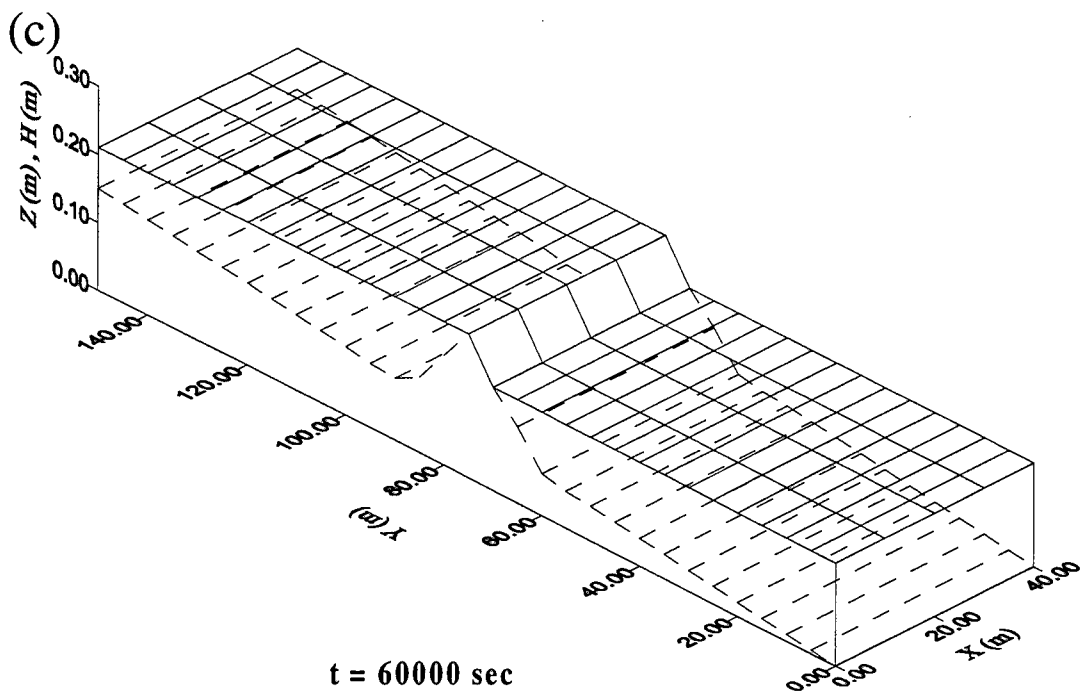
Figure 4.3 Simulated water stage at (b) t = 5,000 sec and (c) t = 60,000 sec for Example 1A
