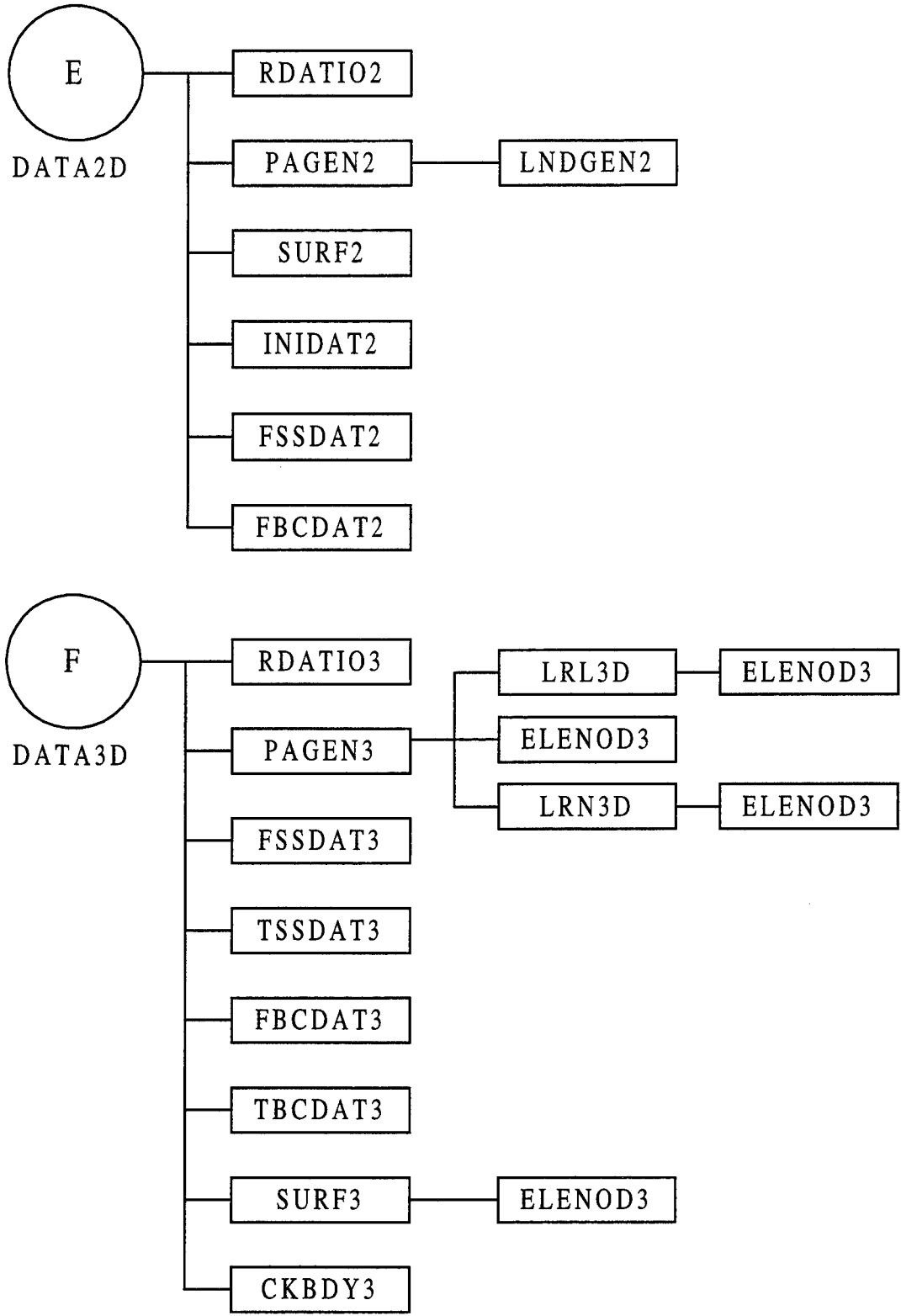
Figure 2.3 Program structure of subroutines DATA2D and DATA3D
