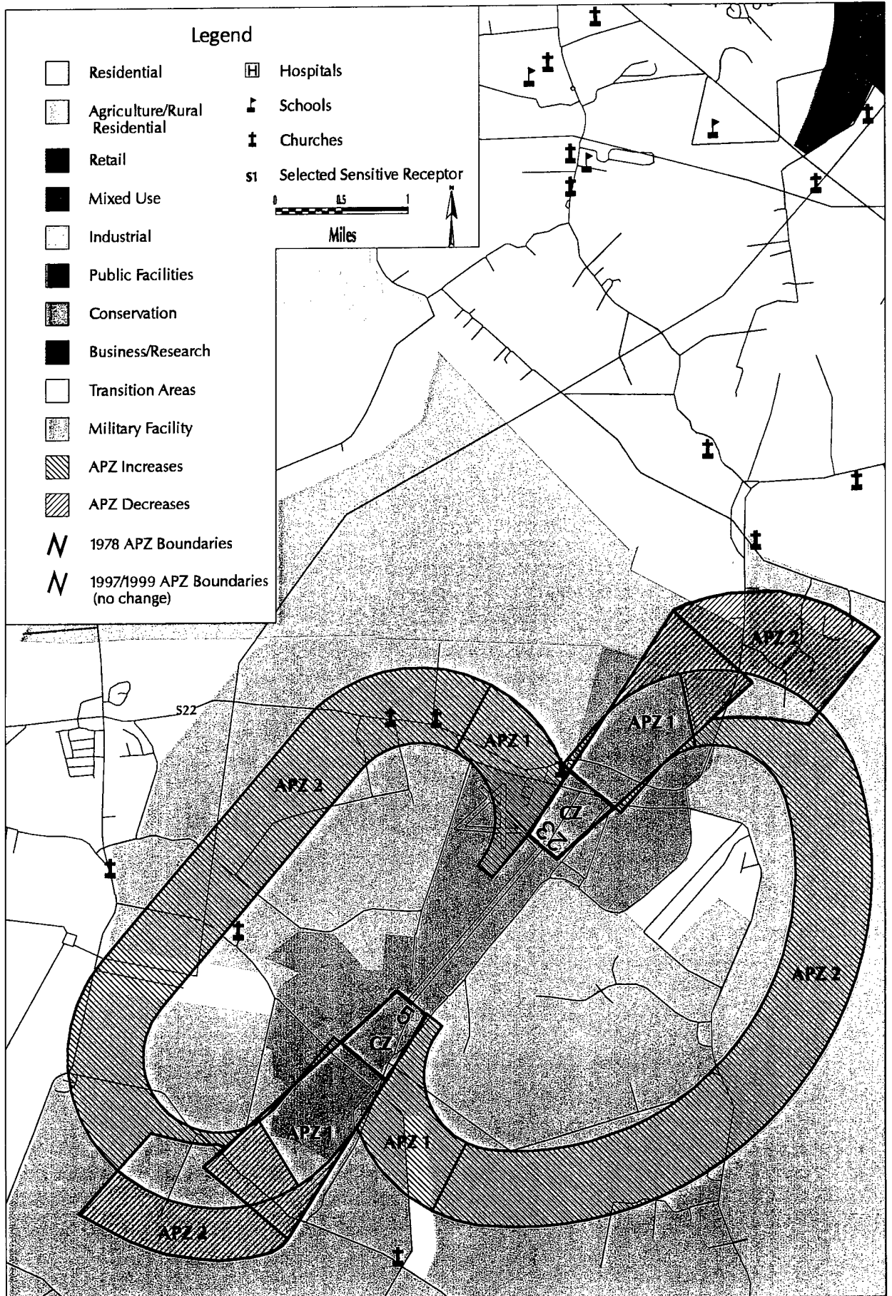
Figure 4.4-6 ARS 1 - Increase/Decrease Between 1978 APZs and 1997/1999 APZs and Land Use NALF Fentress
