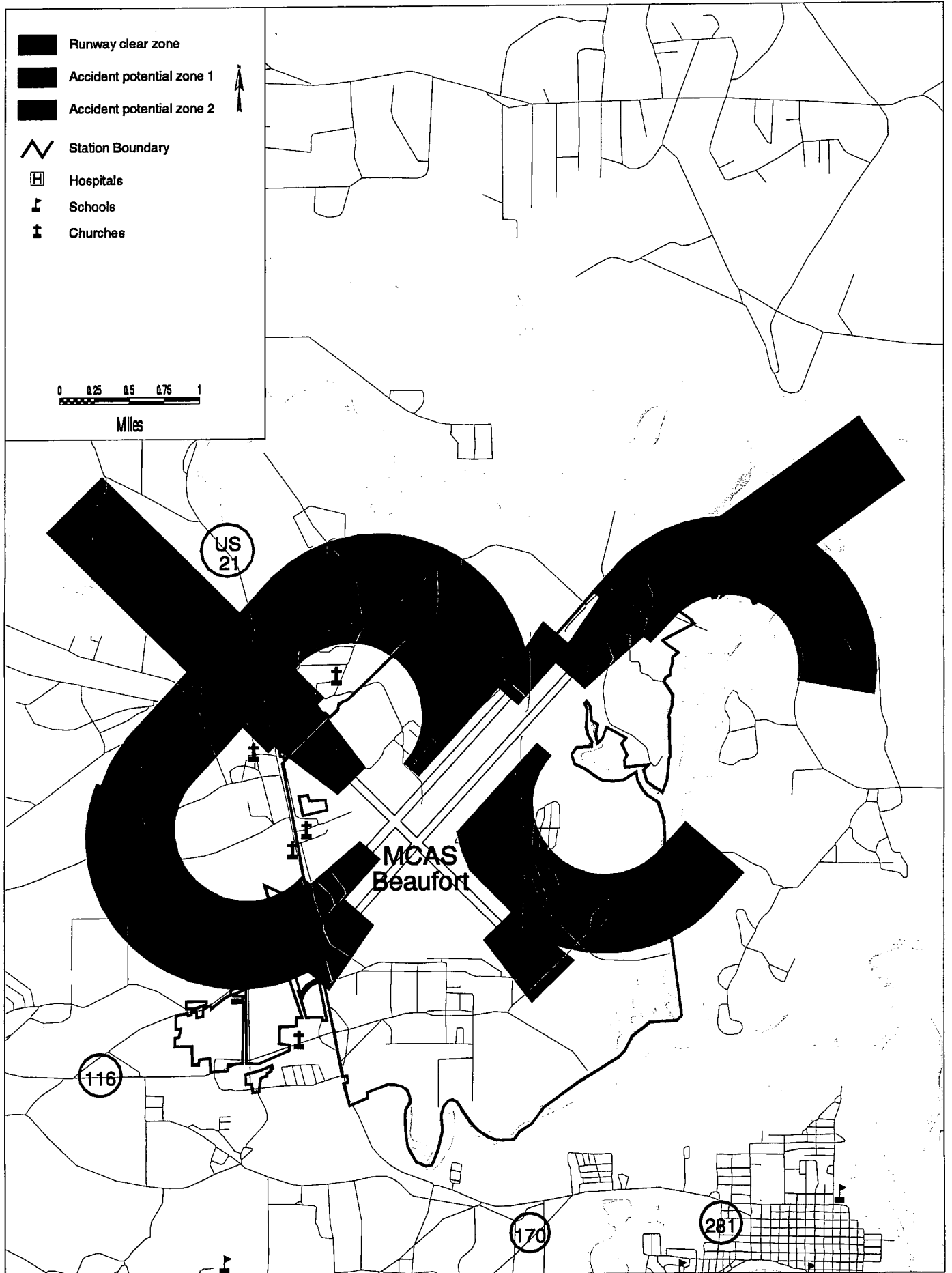
Figure 7.1-2 ARS 4 - Projected 1999 APZs MCAS Beaufort
