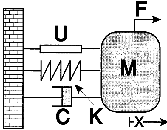
Figure 2.3: An Actuated Structure
