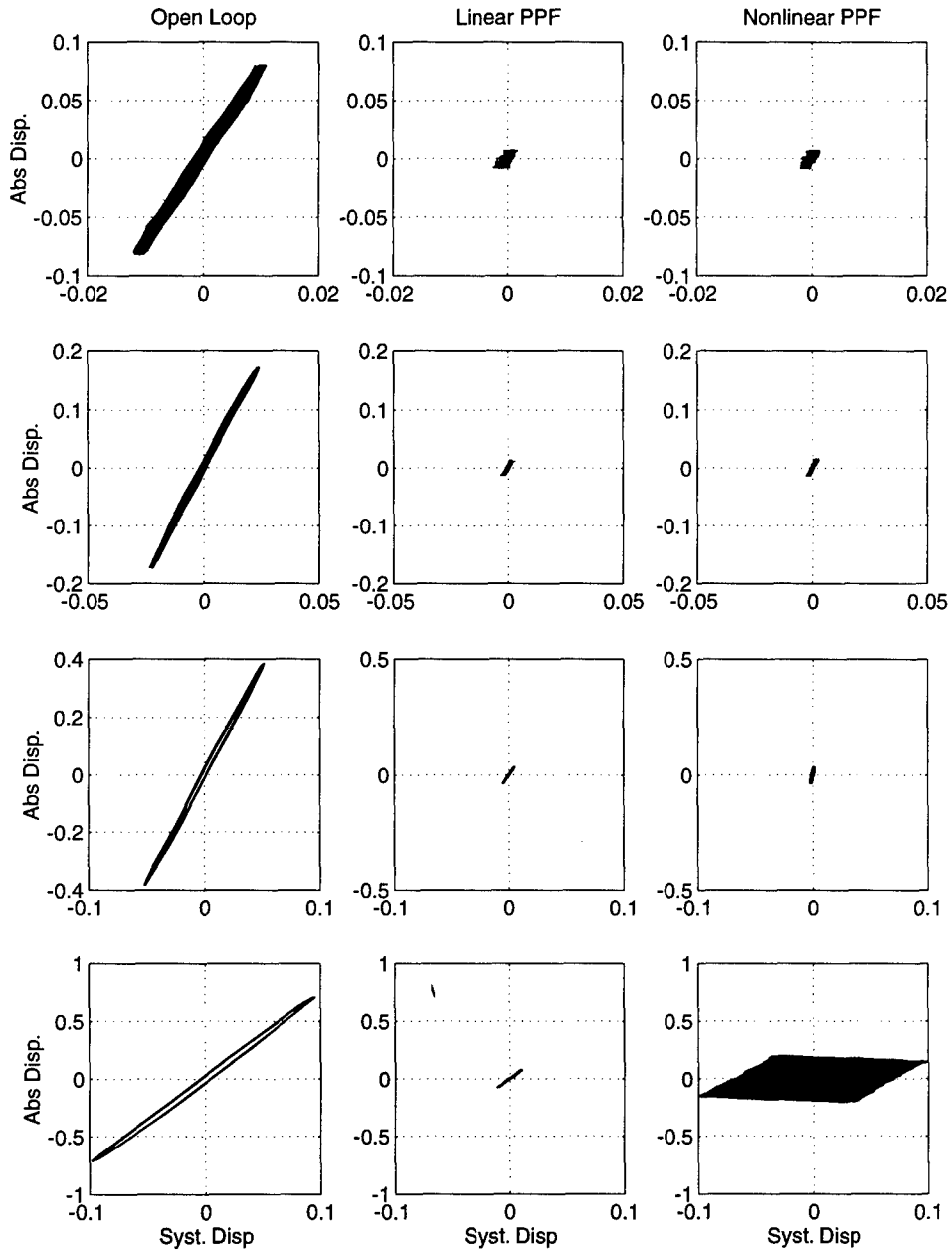
Figure 5.18: Screw Mounted Beam X-Y time response in volts for open-loop, linear and nonlinear PPF controllers. \ddot{x}_0 = 0.005, 0.015, 0.05, and 0.15 g, respectively. X(1) is beam displacement and X(2) is PPF controller displacement. See Appendix B for sensor sensitivities.
