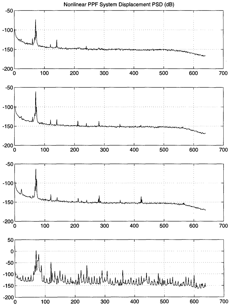
Figure 5.25: Screw Mounted Beam with nonlinear PPF response spectrum for \dot{x}_0 = 0.005 , 0.015 , 0.05 , and 0.15 g.
