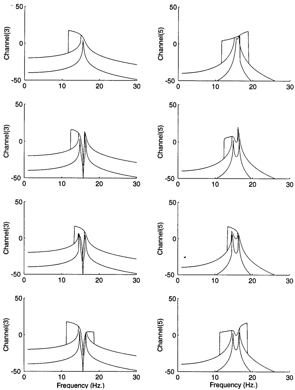
Figure 5.1: Experimental Swept Sine response of the single-degree-of-freedom analog computer experiment. The system (Channel (3)) and absorber response (Channel(5)) are plotted for the open loop, linear absorber, softening absorber, and hardening absorber in rows 1-4.
