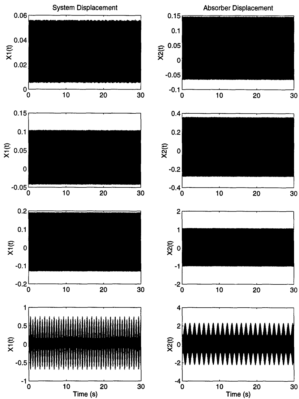
Figure 5.2: Experimental time responses of the single-degree-of-freedom analog computer experiment for f = 0.01, 0.03, 0.1, \text{ and } 0.164 . The system and absorber displacements are plotted in the first and second columns, respectively.
