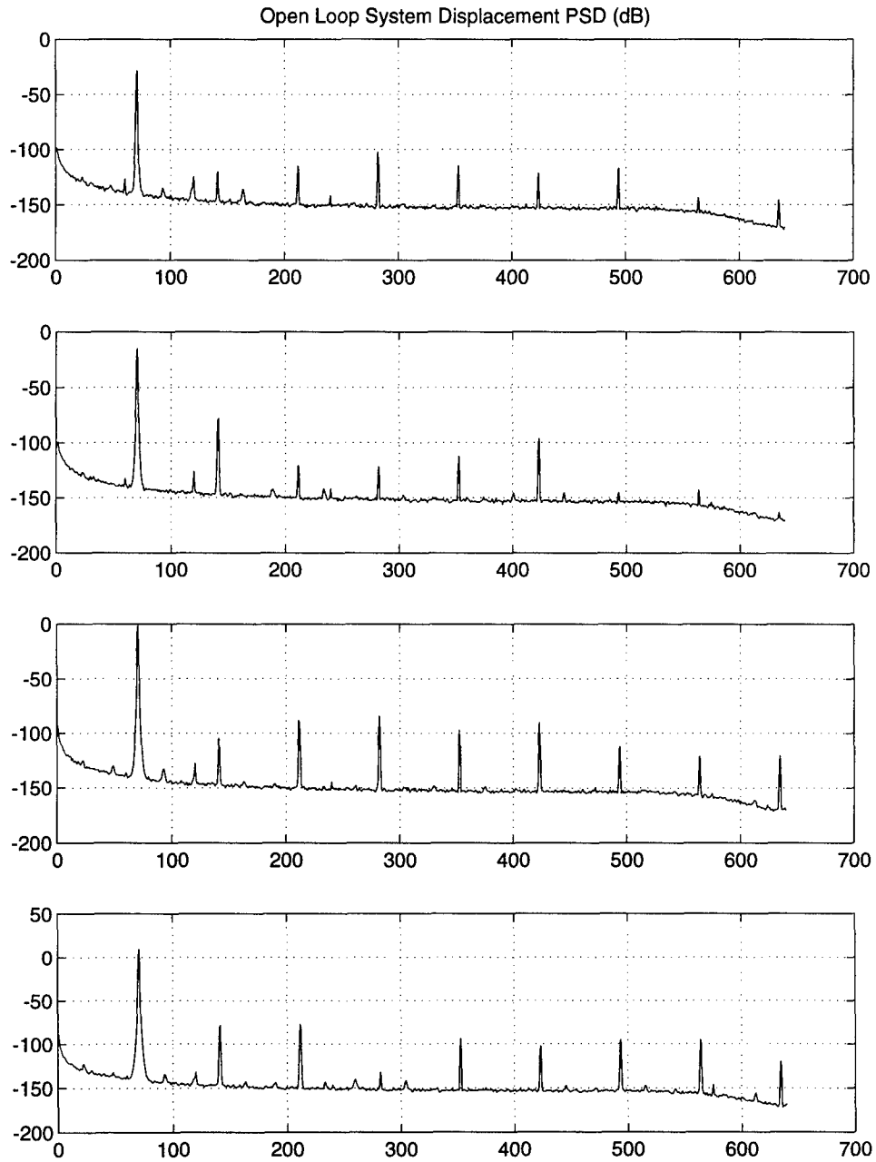
Figure 5.17: Screw Mounted Beam open-loop response spectrum for \ddot{x}_0 = 0.005, 0.015, 0.05, and 0.15 g.
