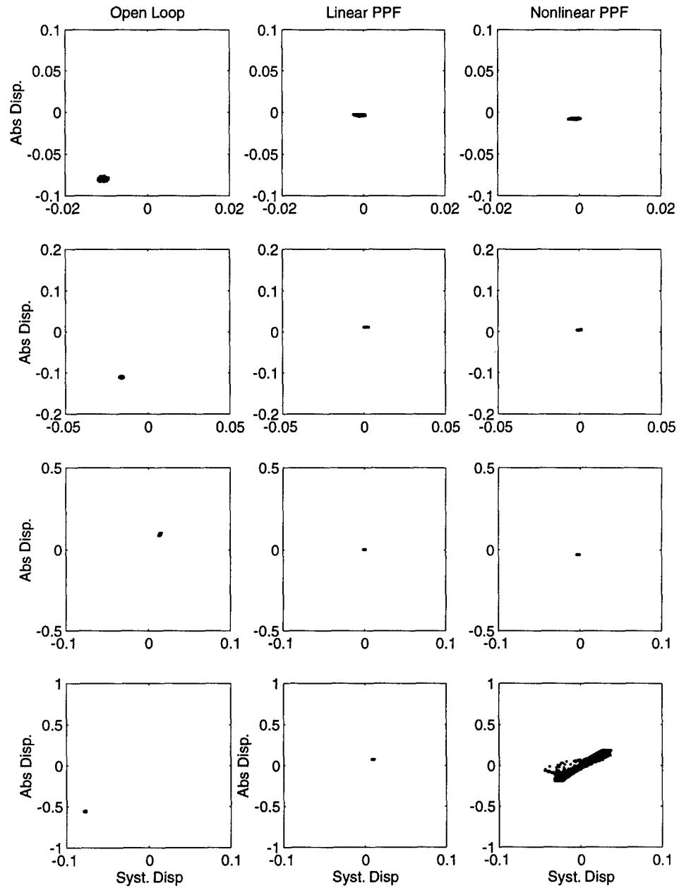
Figure 5.19: Screw Mounted Beam Poincaré sections in volts for open-loop, linear and nonlinear PPF controllers. \ddot{x}_0 = 0.005, 0.015, 0.05, \text{ and } 0.15 \text{ g} , respectively. X(1) is beam displacement and X(2) is PPF controller displacement. See Appendix B for sensor sensitivities.
