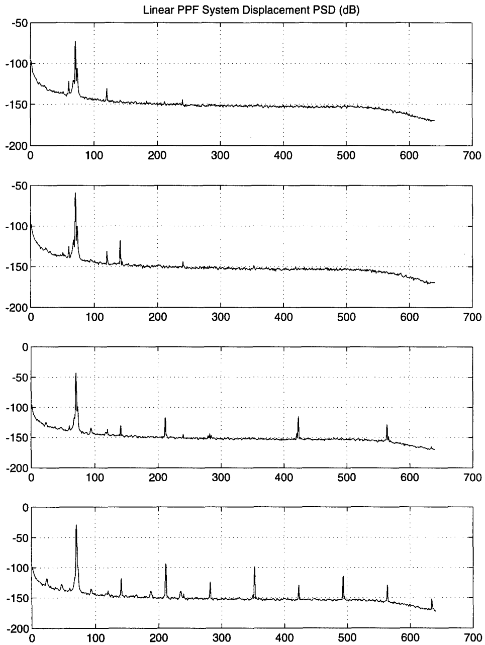
Figure 5.23: Screw Mounted Beam with linear PPF response spectrum for \ddot{x}_0 = 0.005, 0.015, 0.05, \text{ and } 0.15 \text{ g} (from top to bottom).
