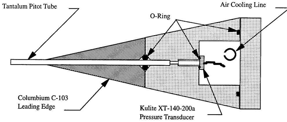
FIGURE 7. CALIBRATION RAKE CROSS-SECTIONAL VIEW
