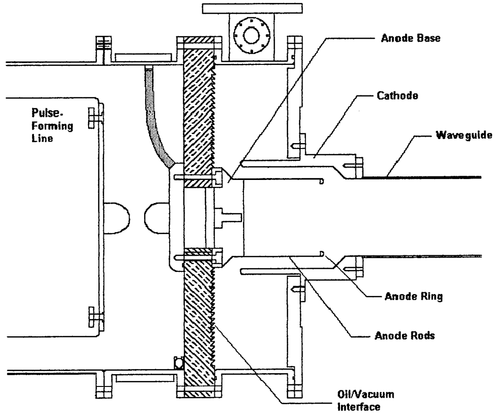
Figure 3: Coaxial vircator installed in the pulsed power system.
