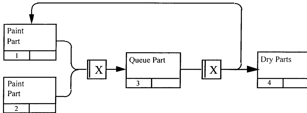
Figure 3-84 Paint/Queue/Dry Process
