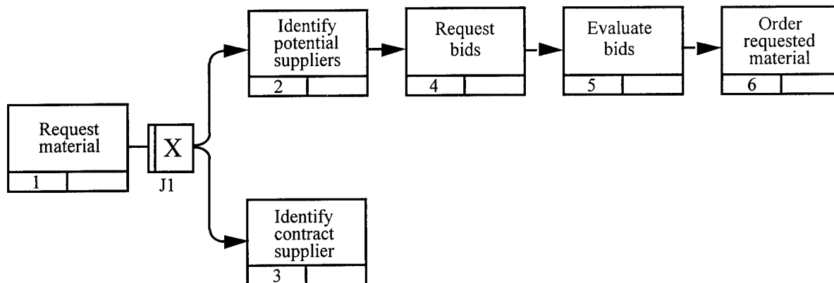
Figure 5-2 Schematic with the First Path Complete
