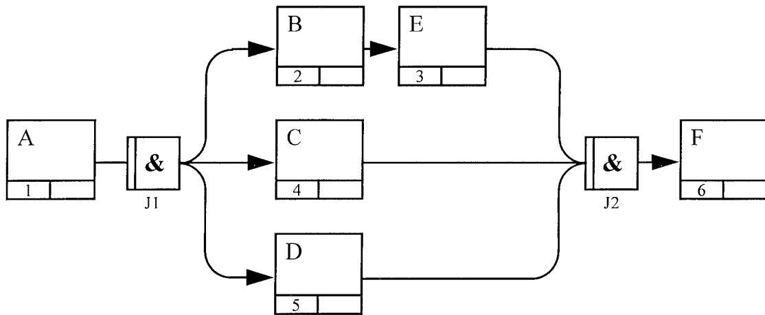
Figure 3-15 Schematic with Asynchronous AND Junctions
