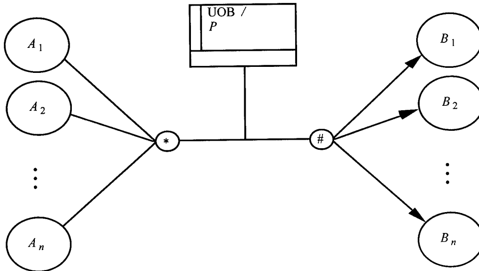
Figure 3-59 Using Multiple Junction Symbols to Display Complex Transition Logic
