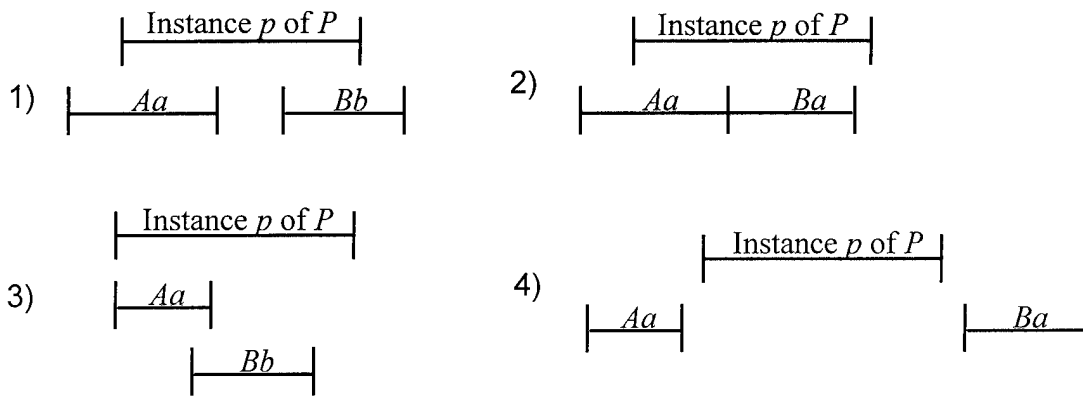
Figure 3-42 Interval Diagrams Representing Instances of Figure 3-41
