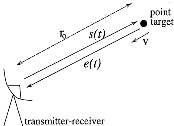
Figure 2.1: Source-Target setup
