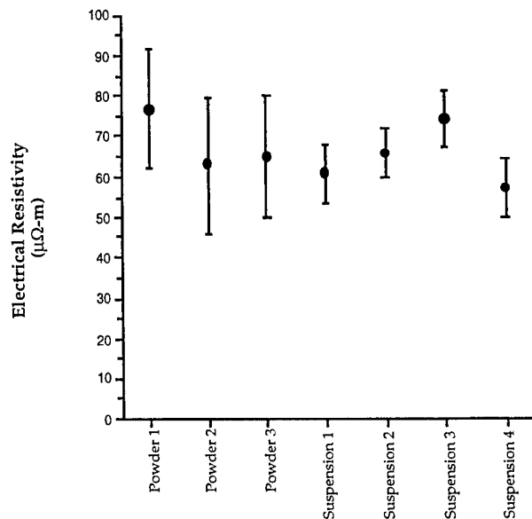
Figure 1: Comparison of carbonized PBO/phenolic carbon/carbon composites by coating method
