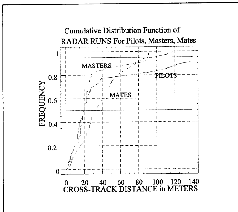
FIGURE 4 - RADAR RUNS
