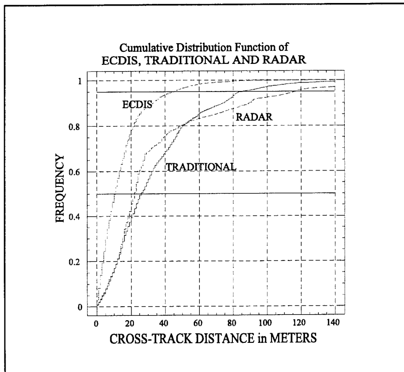
FIGURE 1 - ALL RUNS
