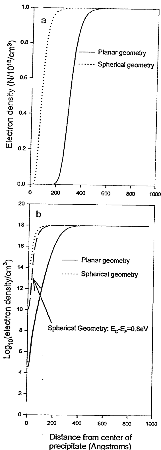
FIG. 15. Comparison of spherical and planar precipitate depletion regions using the DPM with a shallow donor concentration of N_0 = 10^{18}/\text{cm}^3 and a deep trap concentration of N_D^T = 8.84 \times 10^{19}/\text{cm}^3 . (a) Linear scale, (b) logarithmic scale. For the solid and dotted lines E_c - E_f = 0.69 eV, N_D^T/N_A^T = 2 , for the dashed lines E_c - E_f = 0.8 eV, N_D^T/N_A^T = 1.014 .
