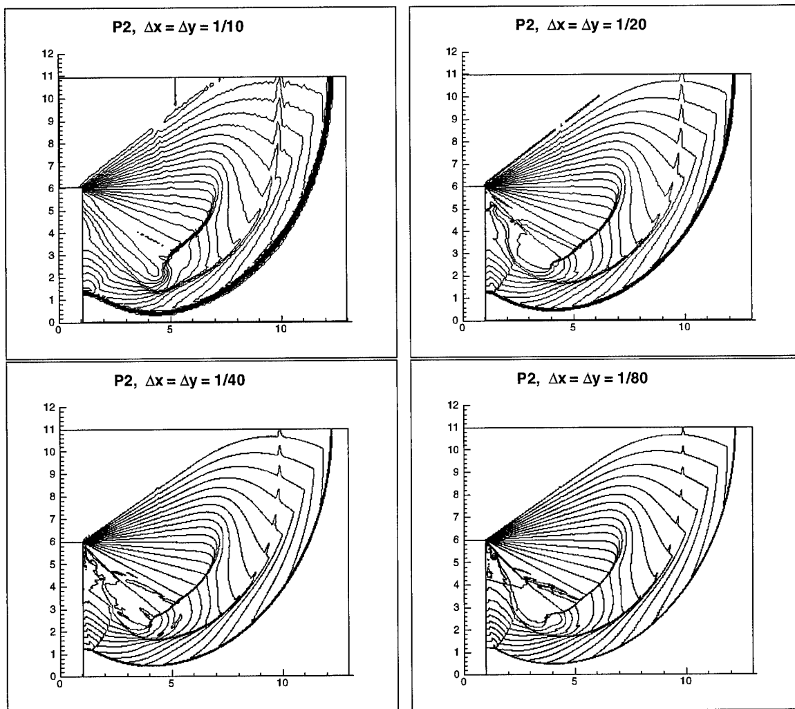
Figure 4.10: Shock diffraction problem. Third order P^2 results. Density \rho . 20 equally spaced contour lines from \rho = 0.066227 to \rho = 7.0668 . Mesh refinement study. From top to bottom: \Delta x = \Delta y = \frac{1}{10} , \frac{1}{20} , \frac{1}{40} , and \frac{1}{80} .
