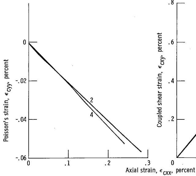
(b) Transverse (Poisson) strain curves.
