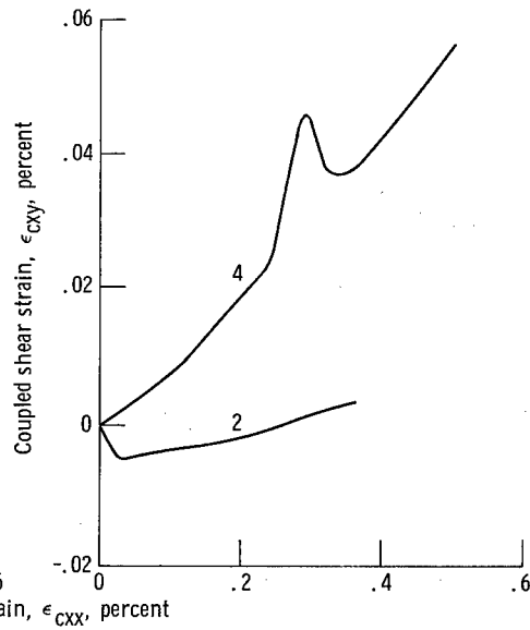
(c) Shear strain curves.
