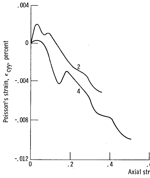
(b) Transverse (Poisson) strain curves.
