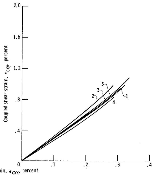
(c) Shear strain curves.
