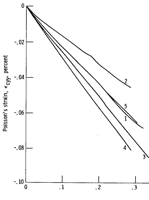
(b) Transverse (Poisson) strain curves.
