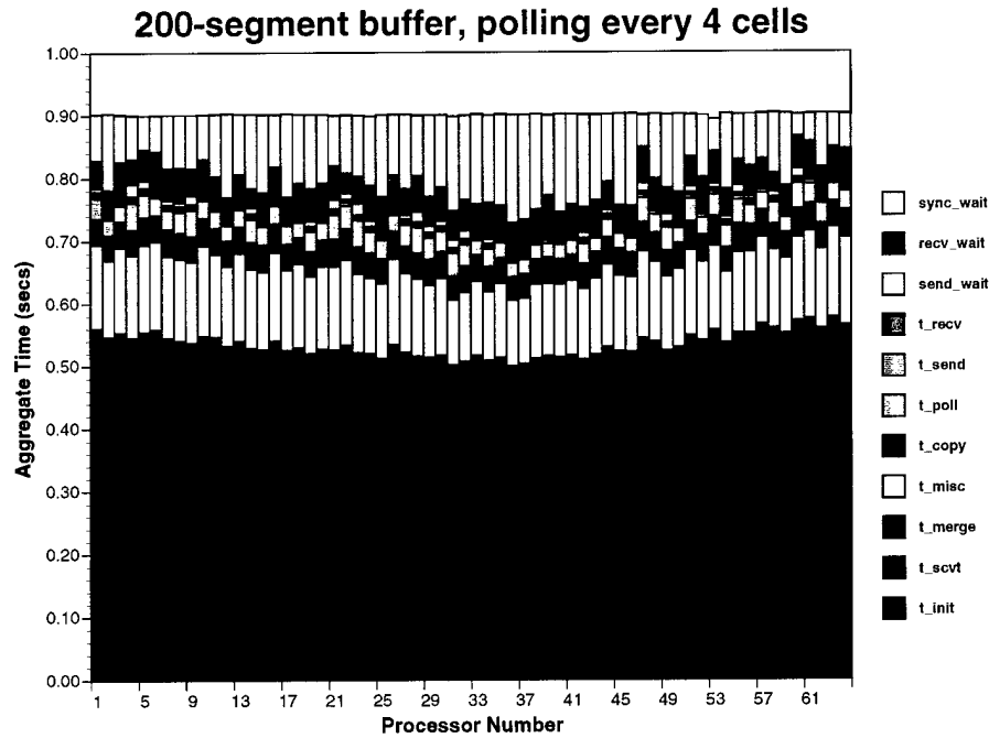
Figure 14: Execution time components for 64 processors; buffer depth = 200, polling after every 4th cell.
