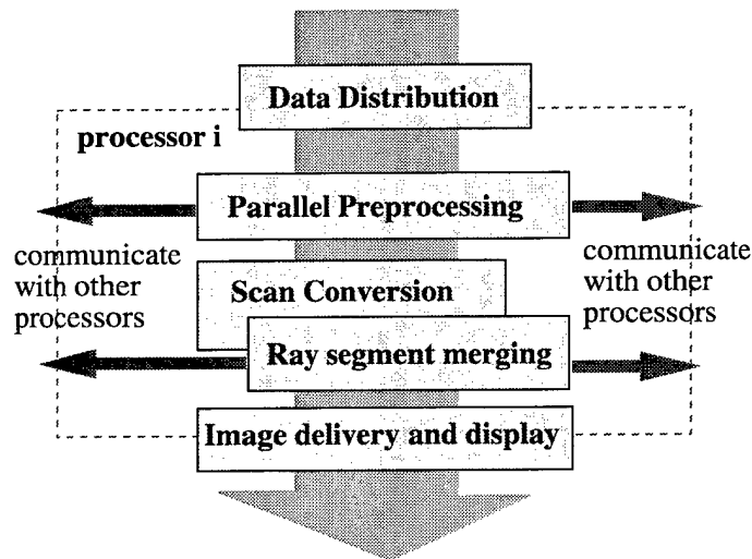
Figure 1: The volume rendering pipeline. This procedure is replicated on every processor.
