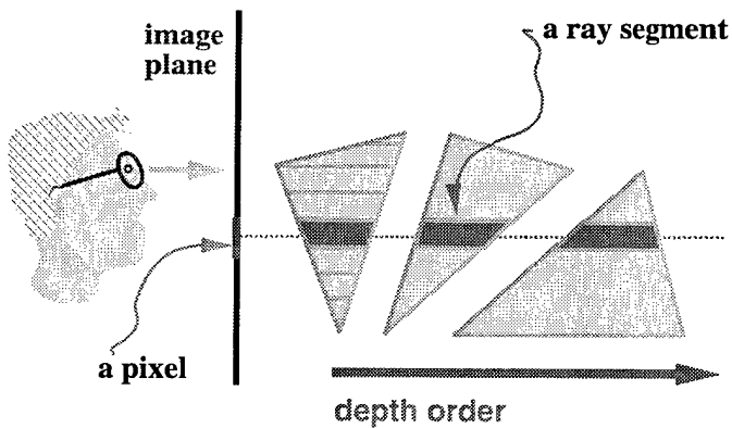
Figure 5: Cell projection rendering.
