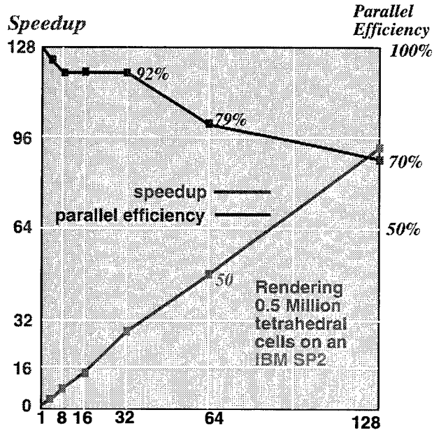
Figure 11: Speedup and parallel efficiency.
