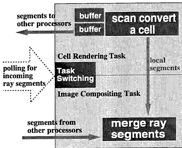
Figure 6: Task management with asynchronous communication.
