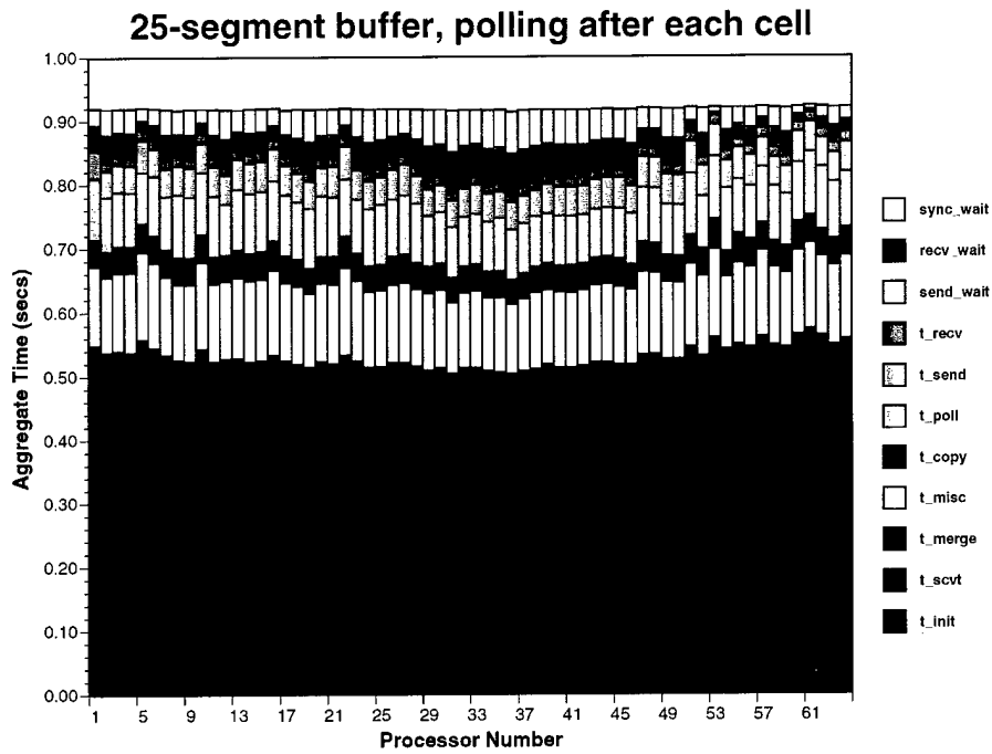
Figure 13: Execution time components for 64 processors; buffer depth = 25, polling after each cell.
