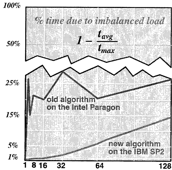
Figure 12: Time delay due to unbalanced load.
