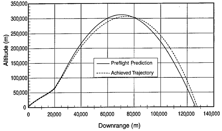
Figure 5.1-1. Comparison of Achieved Trajectory with Preflight Simulation Protection
