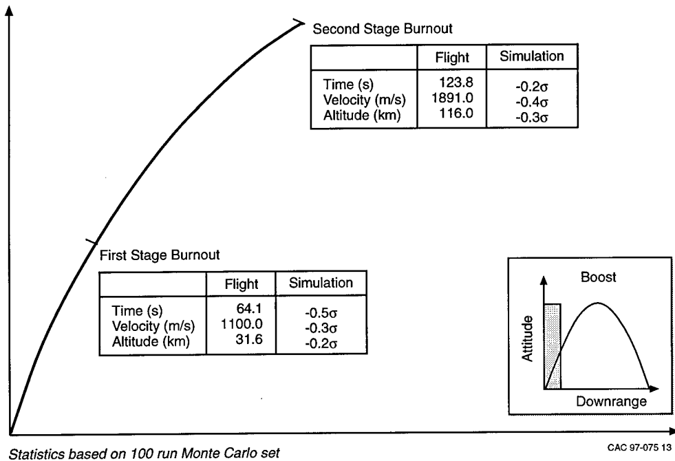
Figure 5.1-2. Overview of Flight 6 Boost Phase Performance
