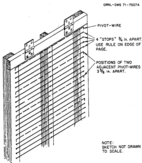
Fig. 11. Positions of pivot-wires and flap-stops.
