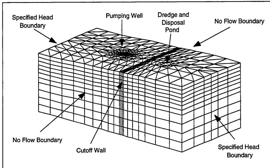
Figure 12. Groundwater remediation application showing numerical model mesh and assigned boundary conditions
