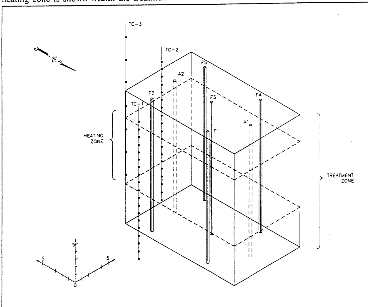
Figure 14 Isometric view of applicator and monitoring wells.
