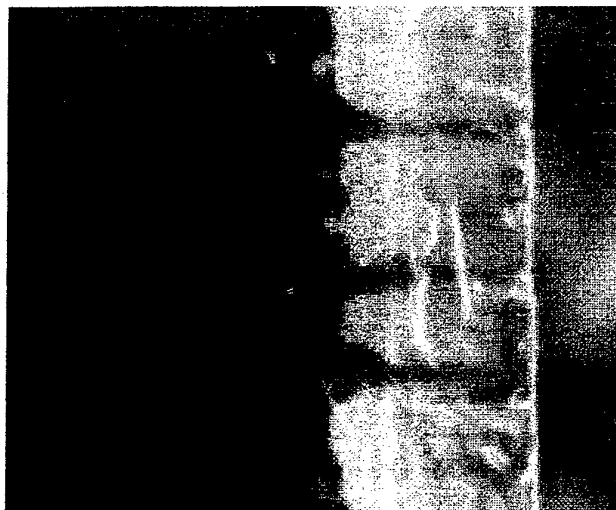
Fig.2.5 Real CCL - SEM image of cross-section of the GaN epilayer grown on SiC substrates (0.3 mm thickness). Blue stripe is interface layer between substrate (at the left) and grown GaN-epilayers (at the right).
