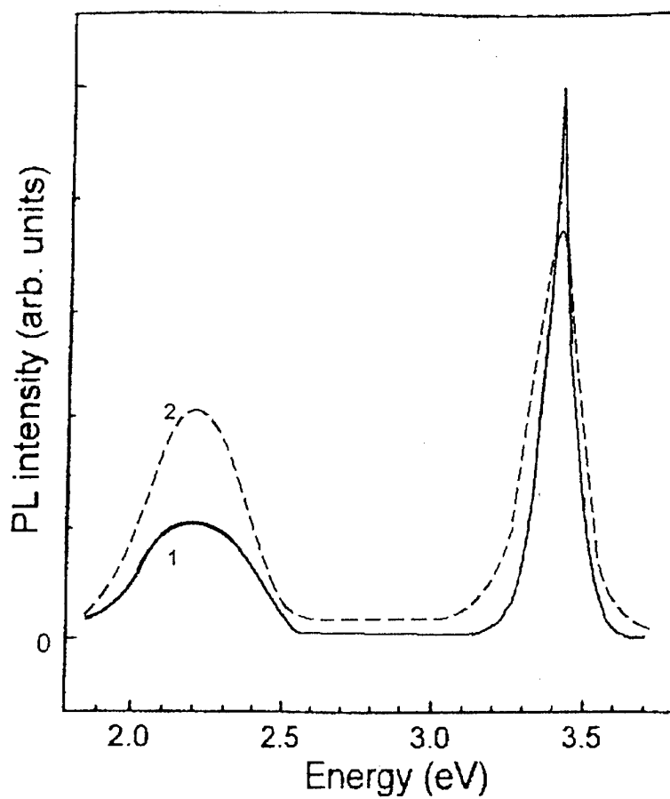
Fig. 2. 3 Photoluminescence spectra at room temperature for two GaN epilayers grown on SiC substrates at different temperatures ^{\circ}\text{C} ; 1140 - solid curve; 1210 - dotted curve.
