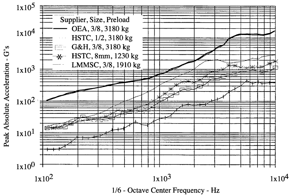
Figure 7. Device comparison, LMMSC panel simulator with masses, SRS ( \phi=10 ), 95th percentile levels.
