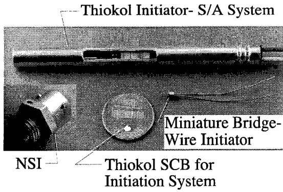
Figure 10. Thiokol miniaturized, programmable delay, SCB, electro-optical S/A and initiation system.
