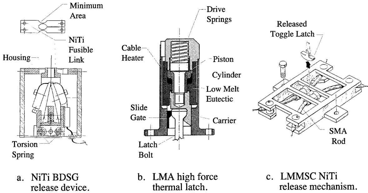
Figure 4. NEA release mechanisms.
