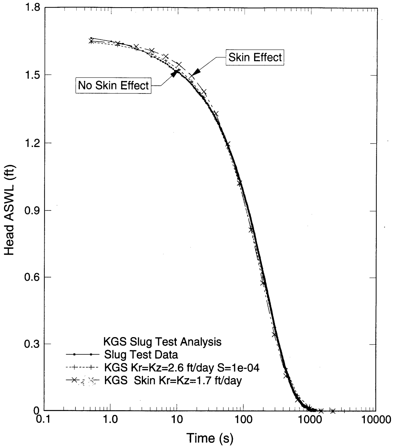
Figure 35. Comparison of Slug Test Data to KGS Model Calculations Conducted With and Without Low Permeability Skin Effect. Calculation Without the Skin Effect Is a Better Match to the Slug Test Data.
